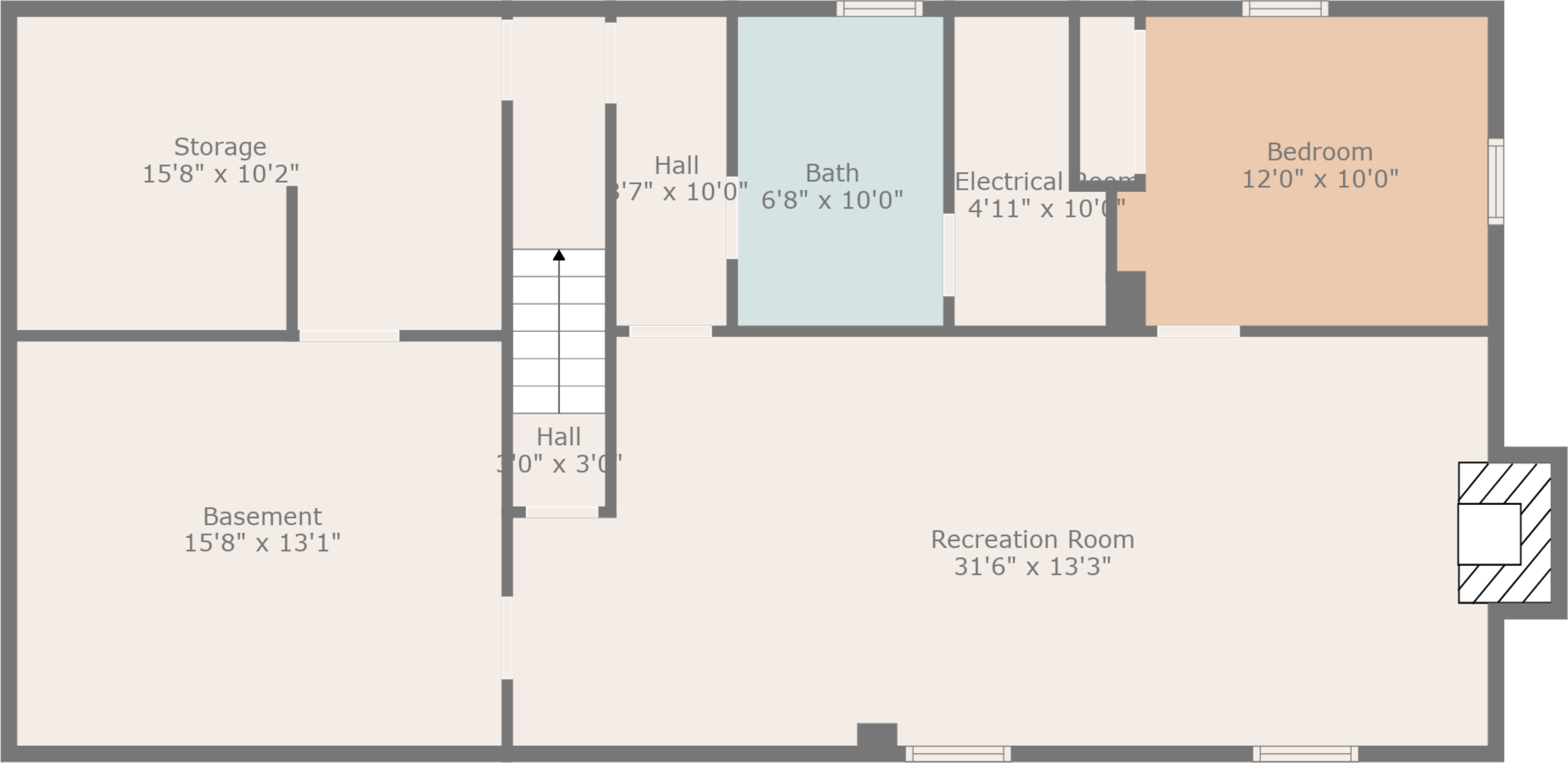
Floor 1
