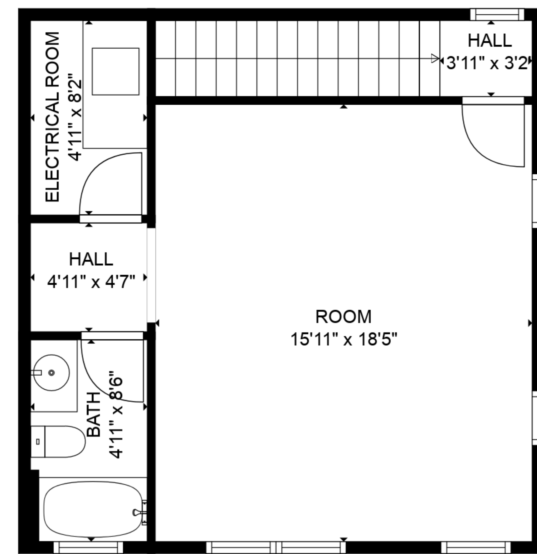
FLOOR 2
