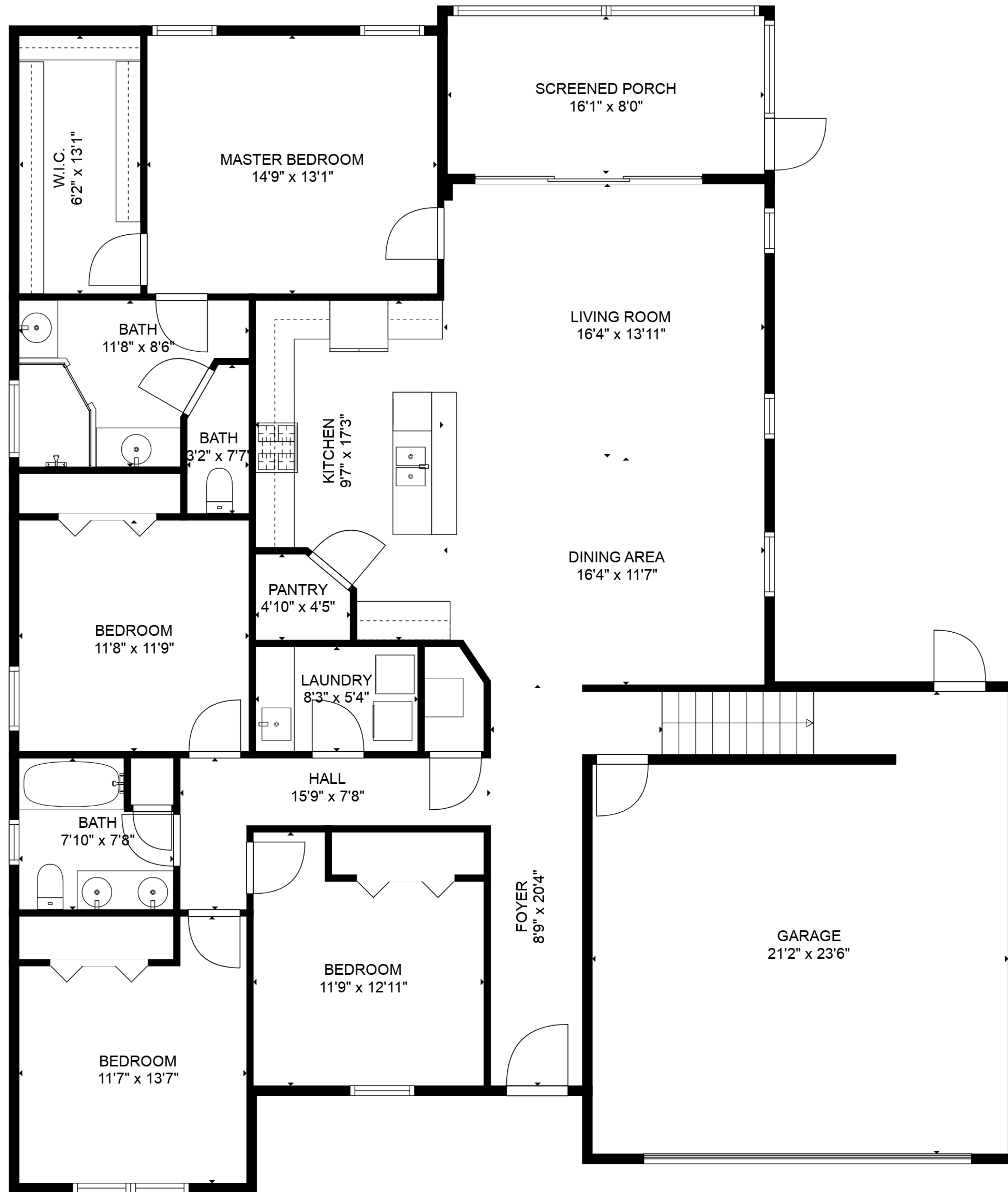
FLOOR 1
