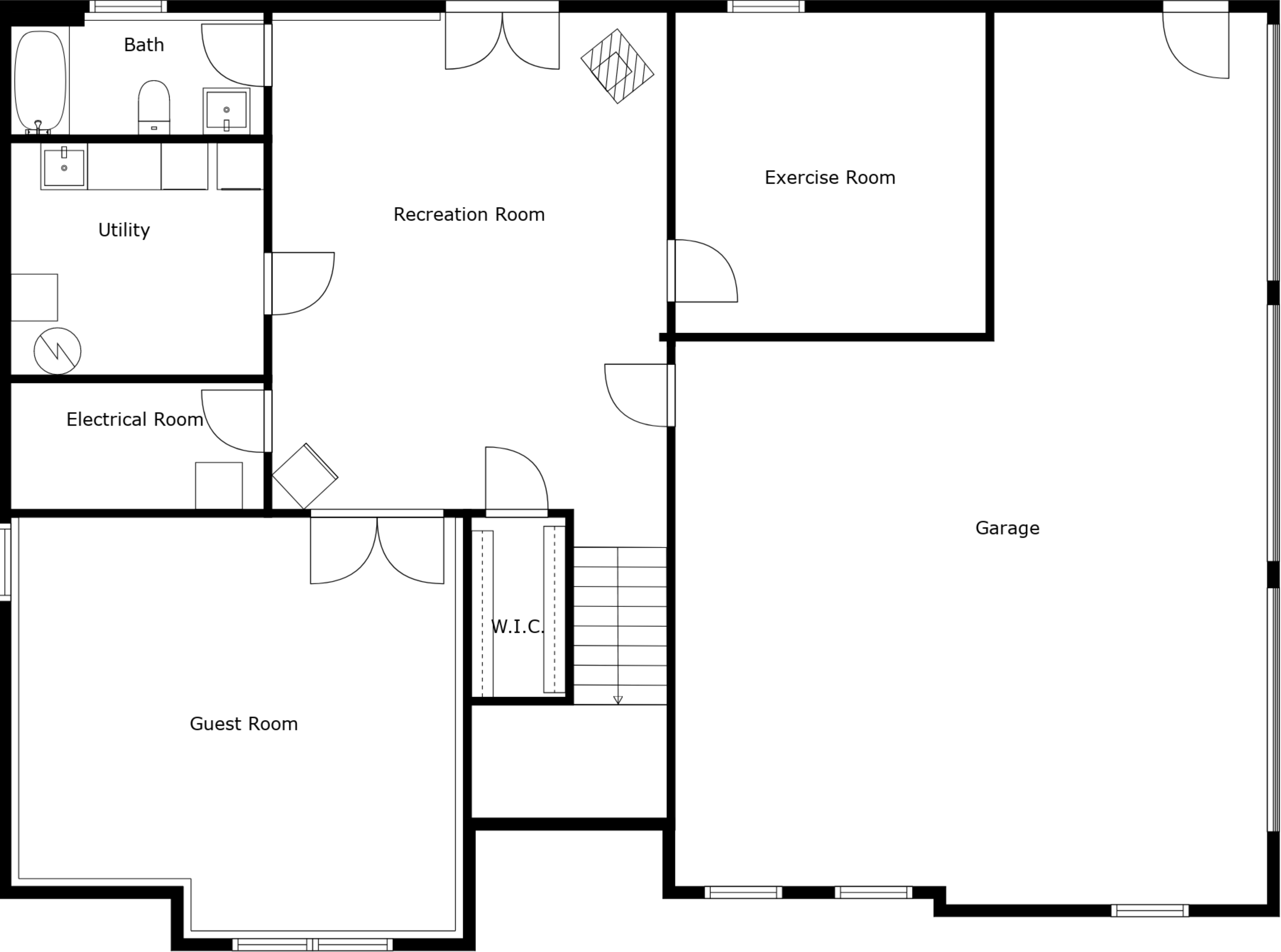
Floor 1
