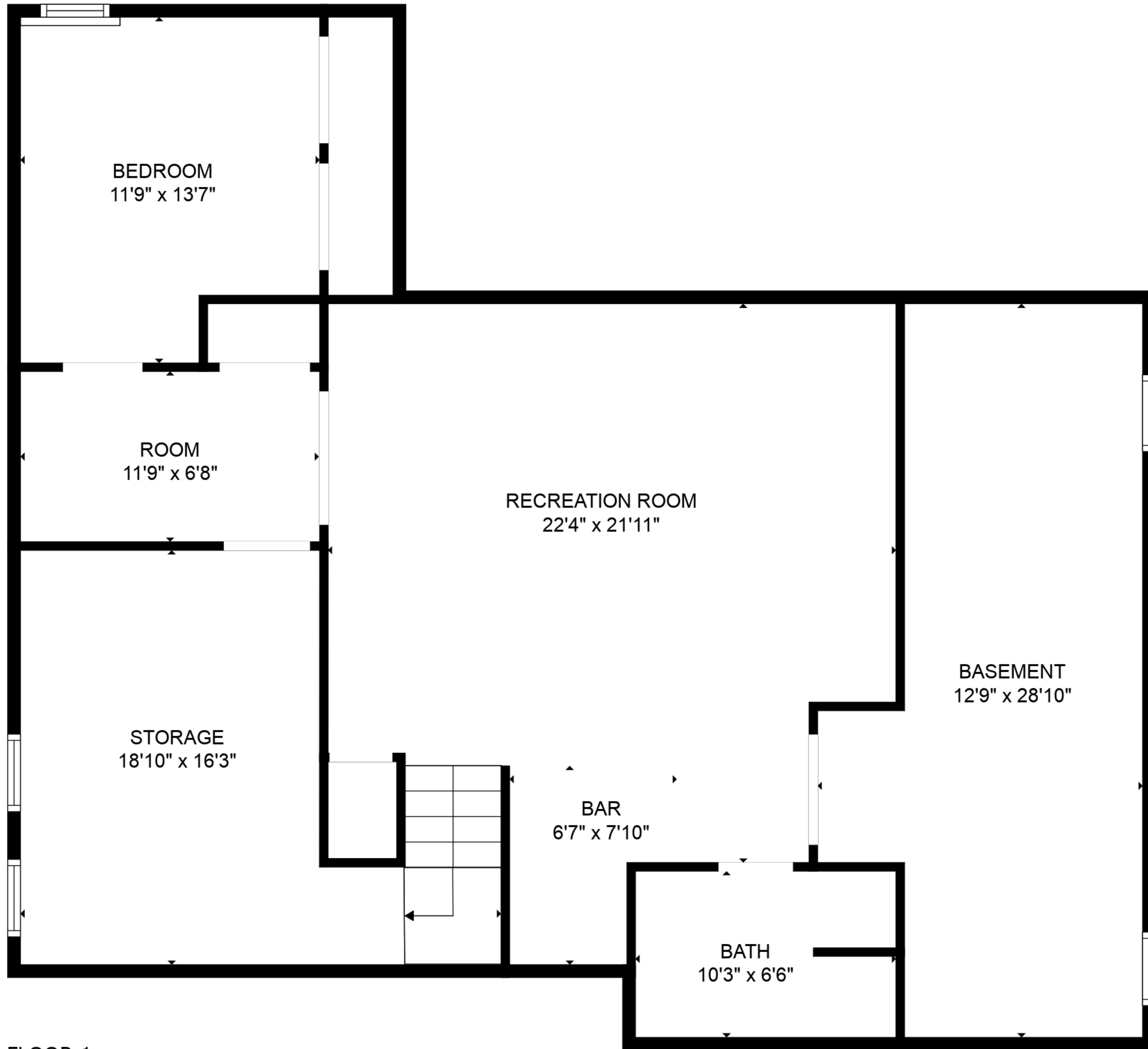
FLOOR 1
