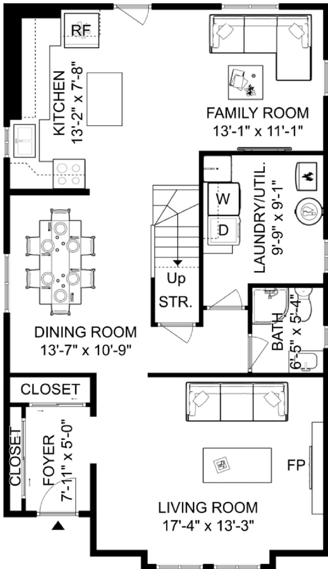
MAIN FLOOR 1,079 sq.ft. | Ceiling Height: 8'-0"
