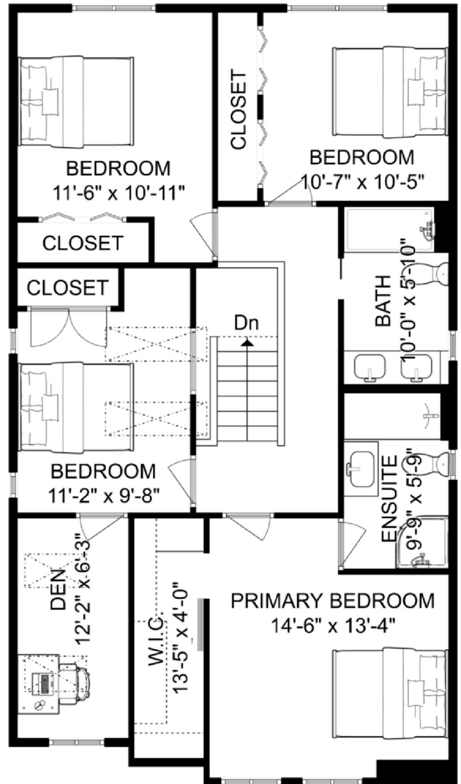
UPPER FLOOR 1,077 sq.ft. | Ceiling Height: 8'-0"
