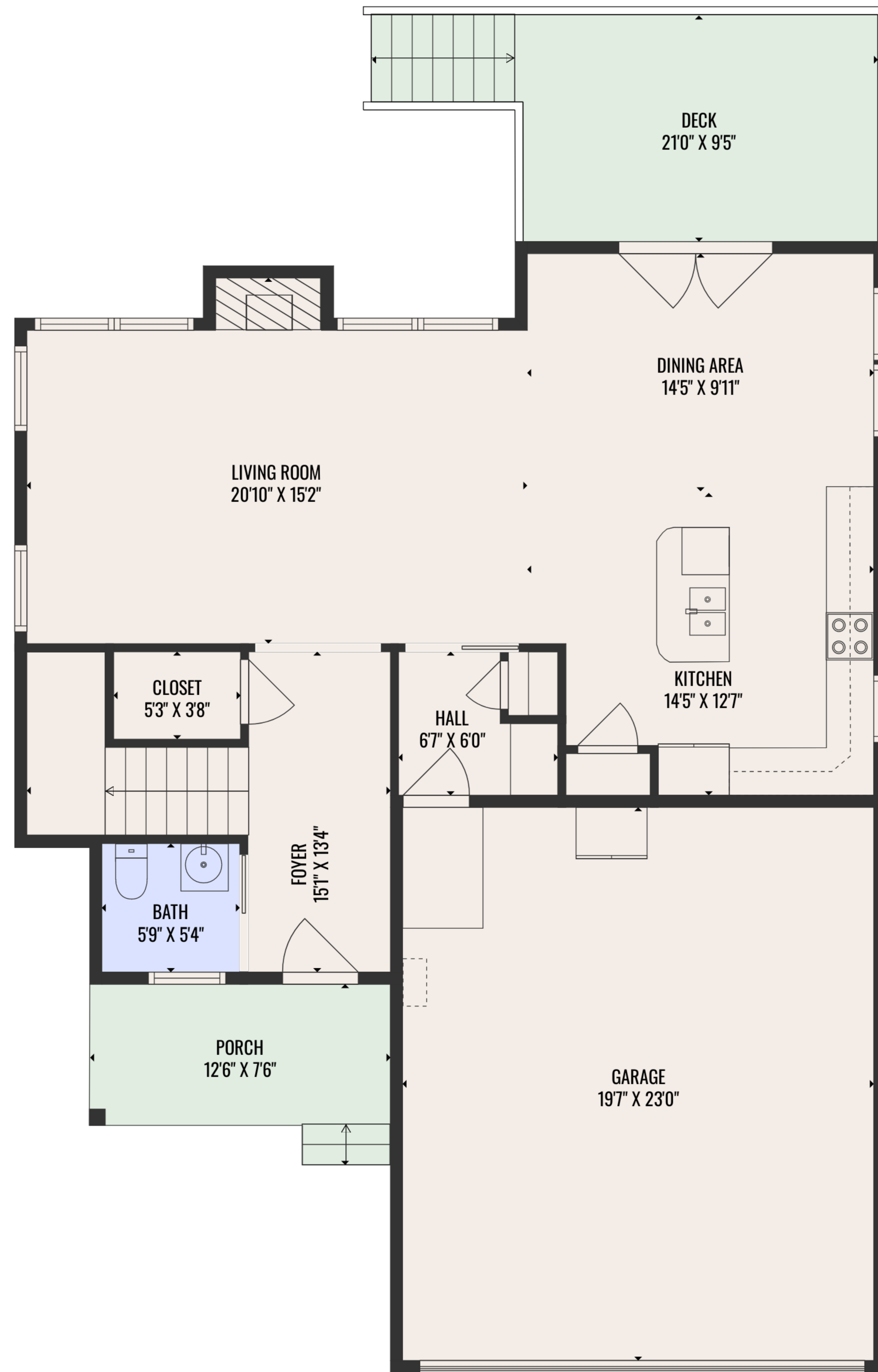
FLOOR 1
