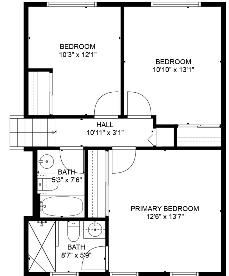
FLOOR 3
