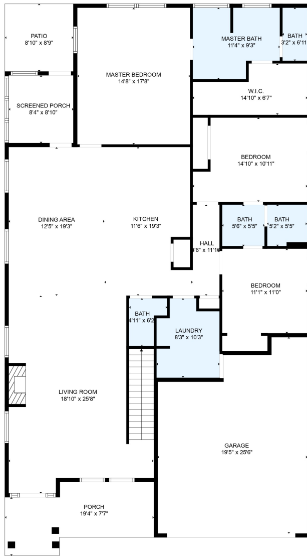
FLOOR 1
