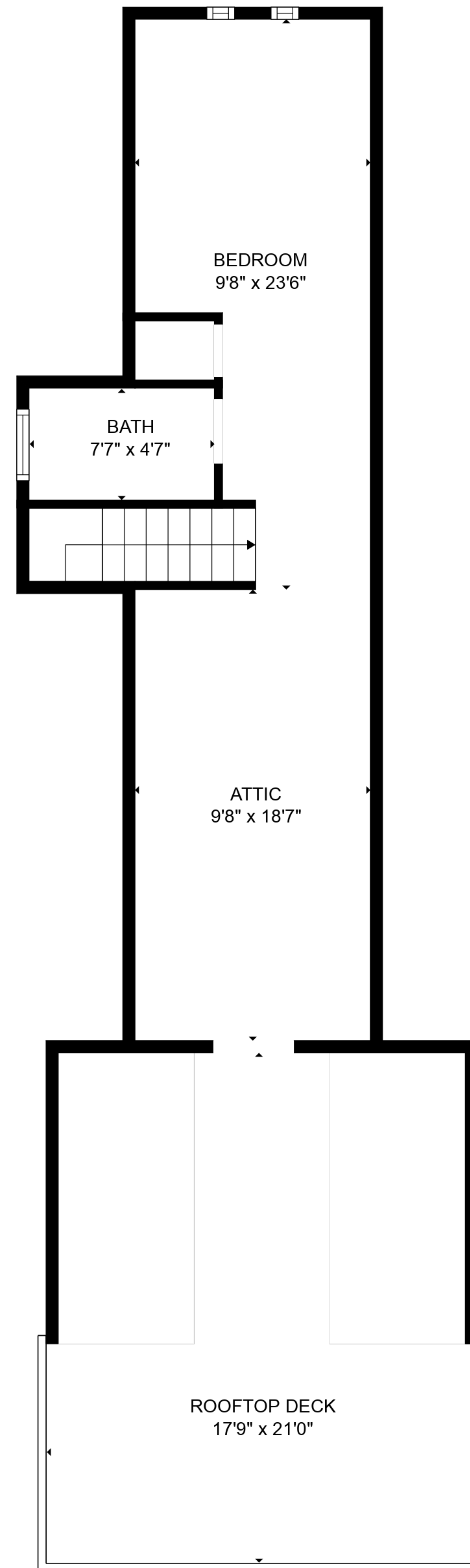
FLOOR 2
