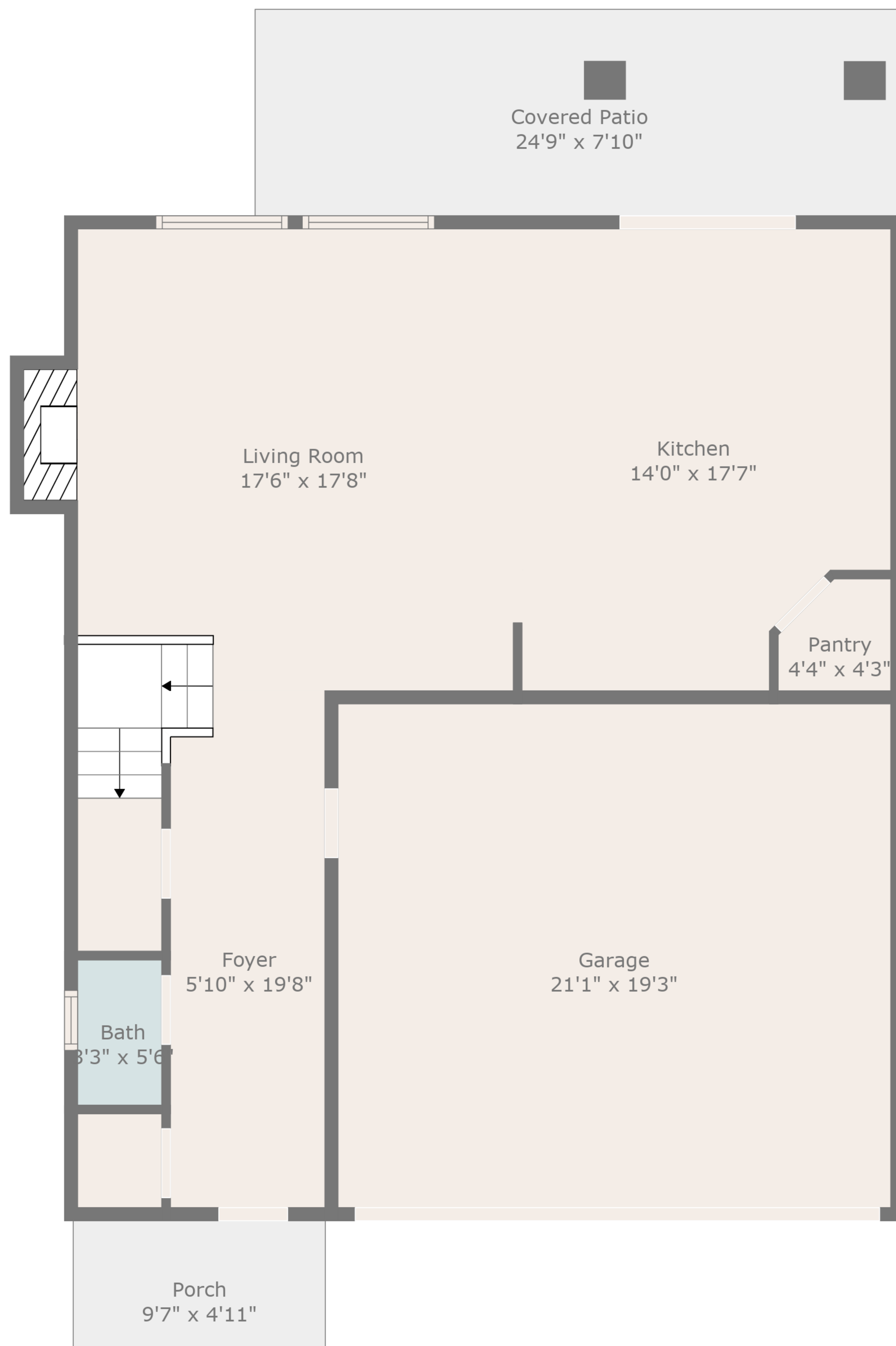
Floor 1
