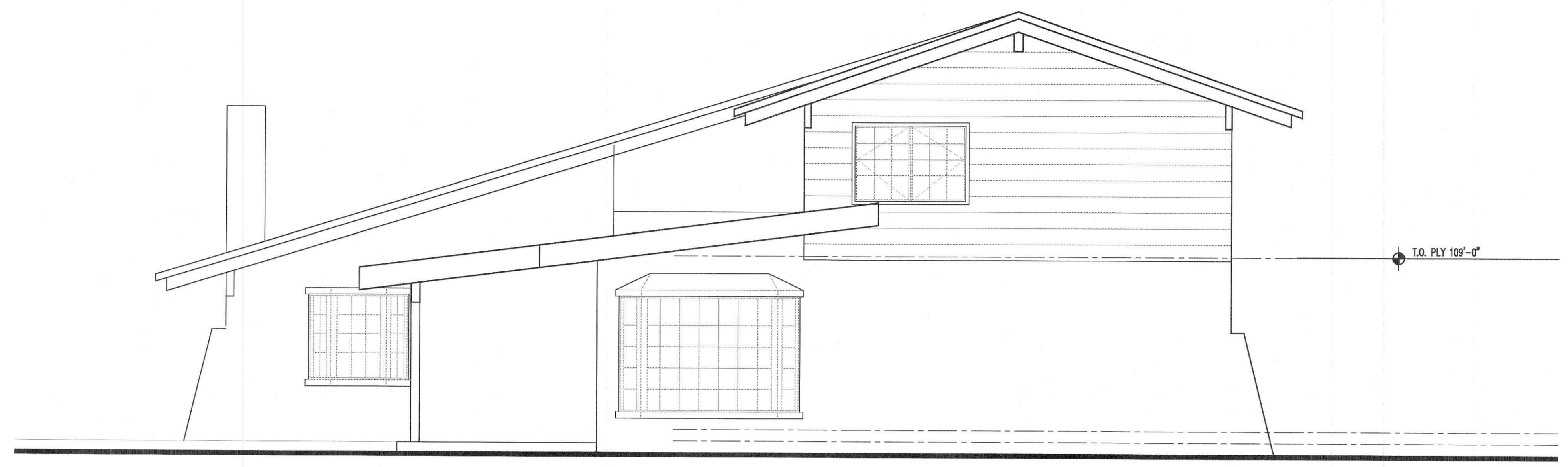
1 PROPOSED NORTH ELEVATION A3.1 1/4" = 1'
