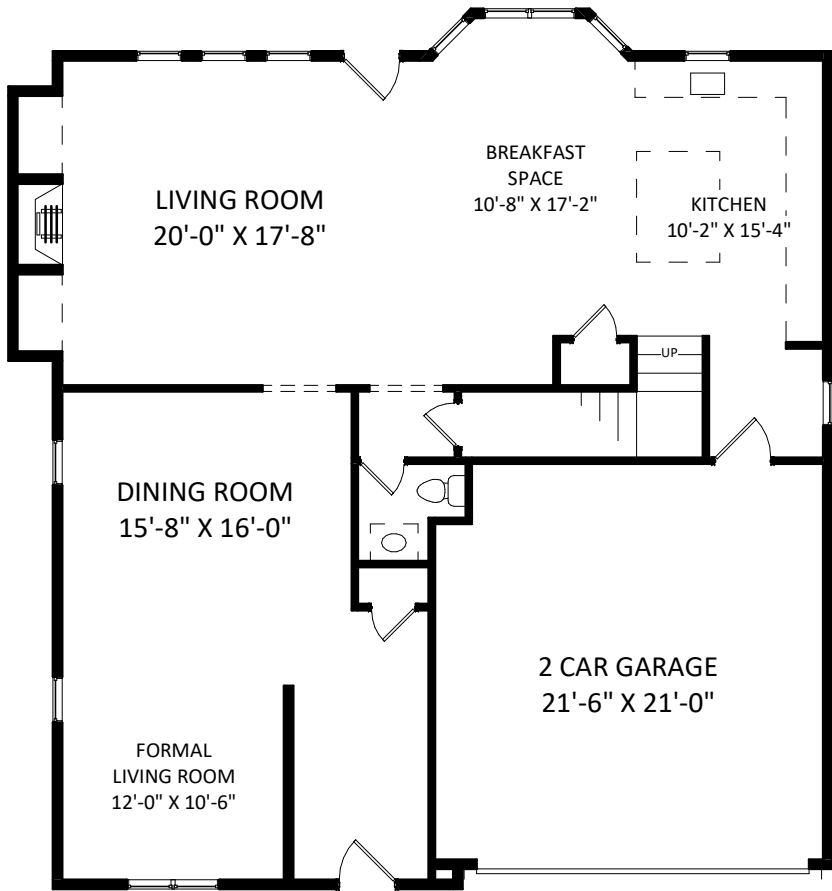
1st FLOOR
