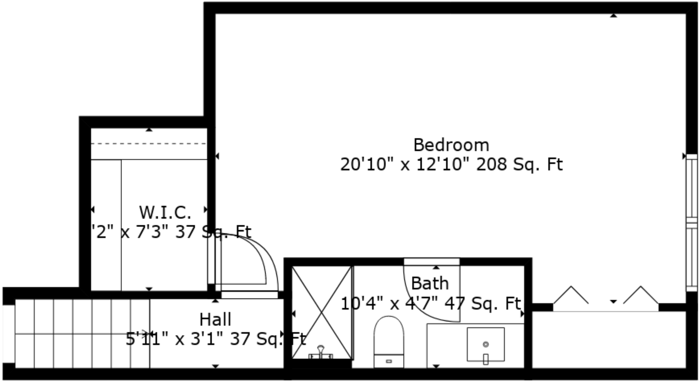
Floor 3
