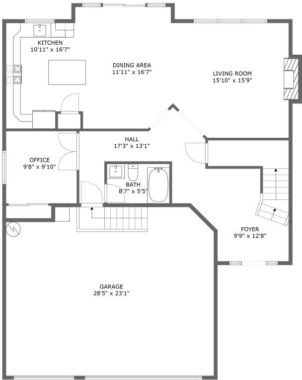
FLOOR 1
