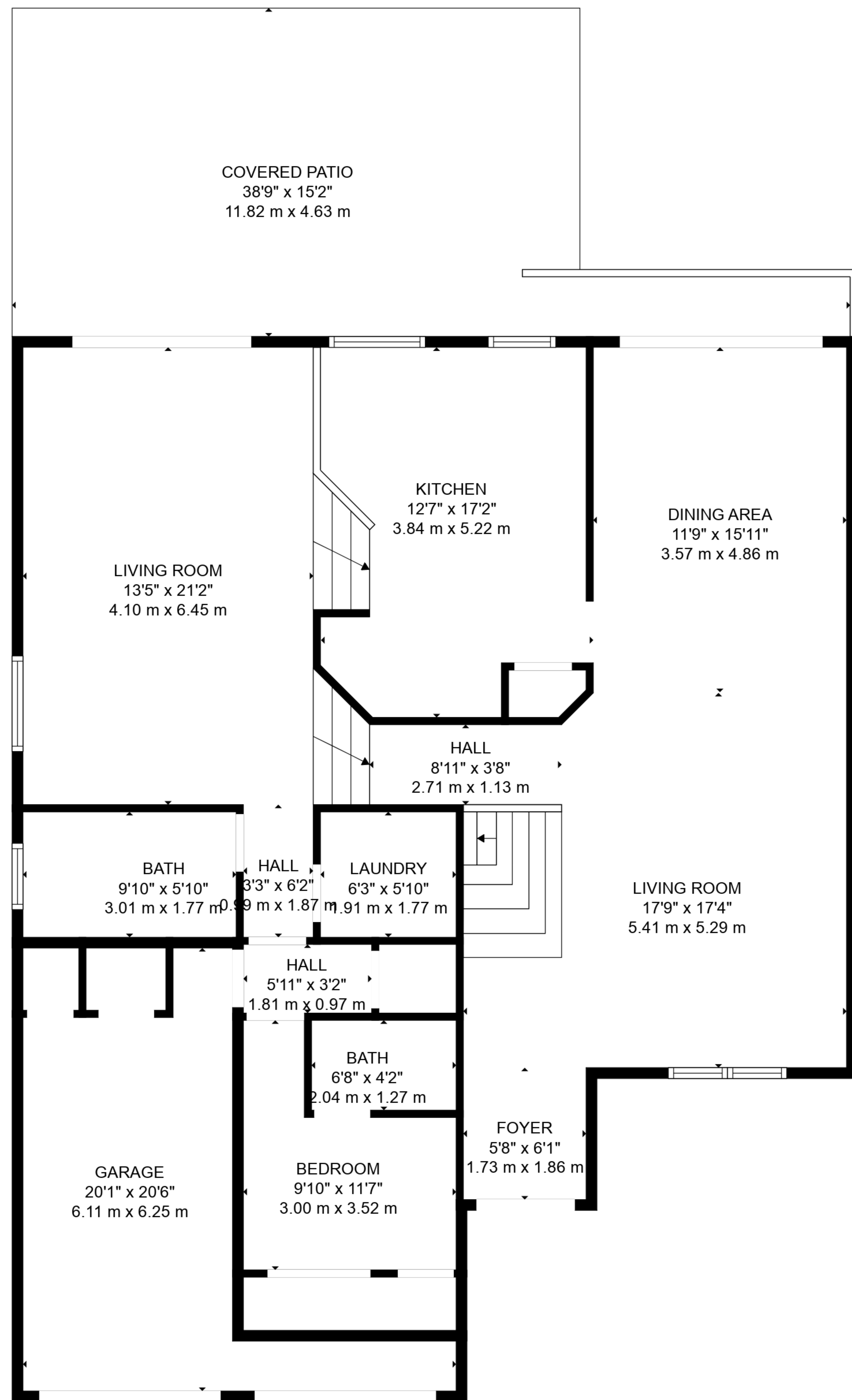
FLOOR 1
