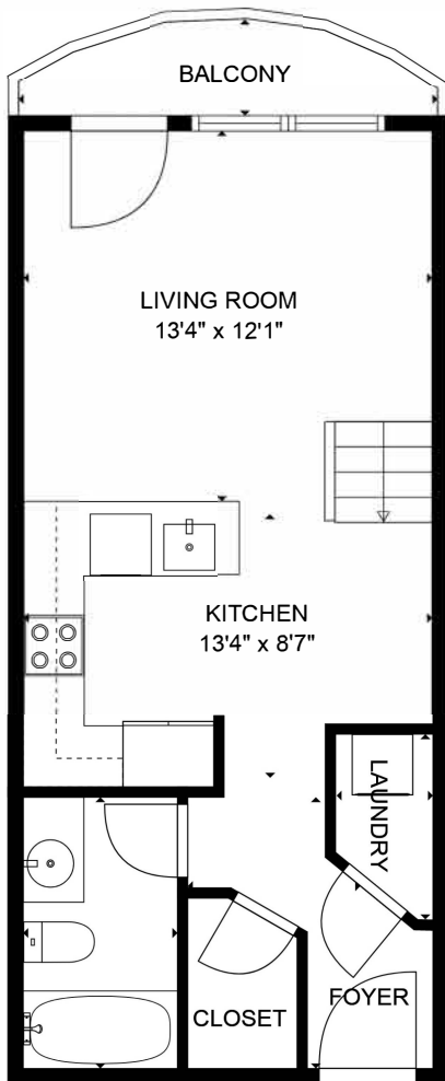
MAIN LEVEL
