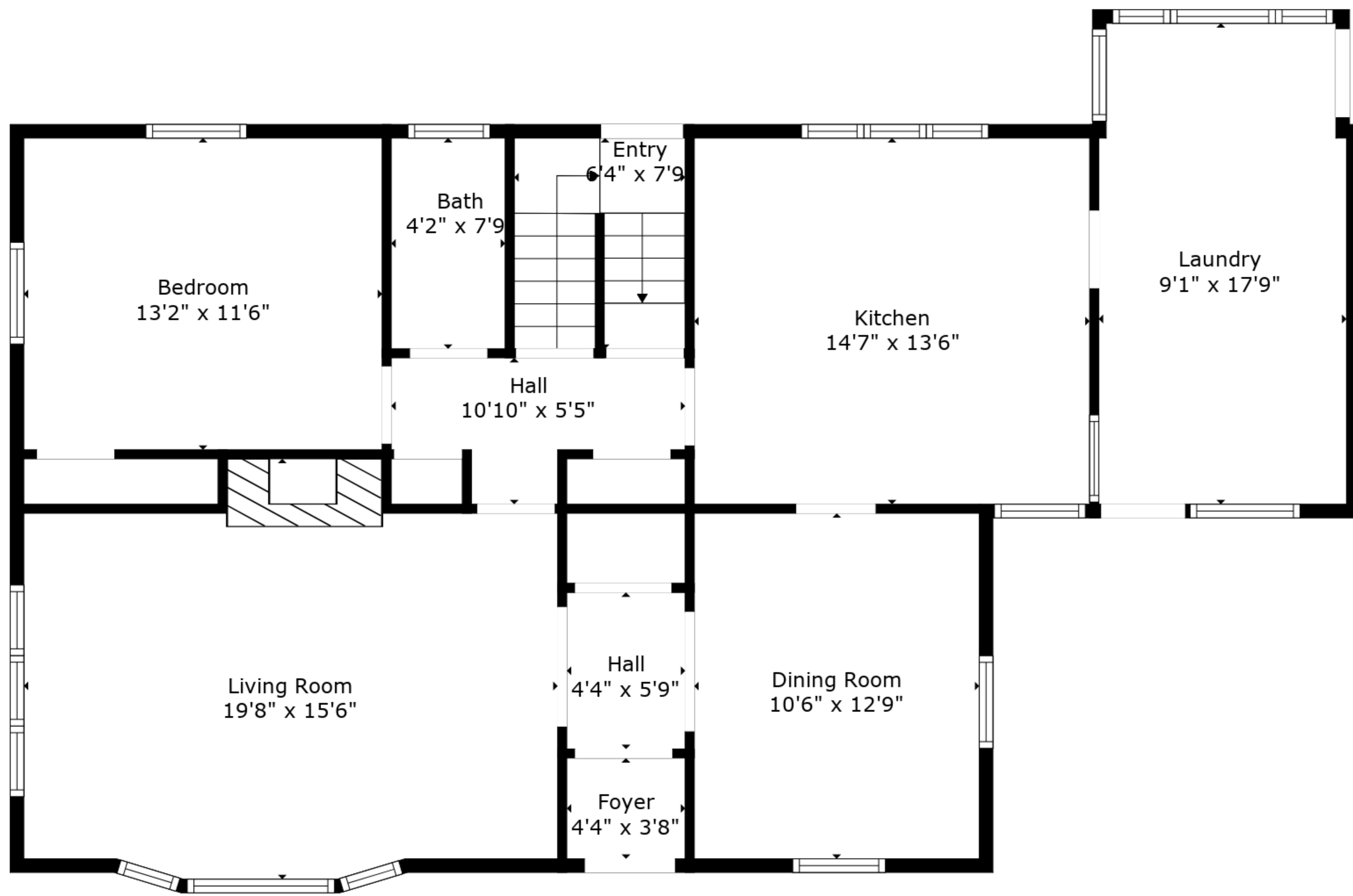
Floor 2
