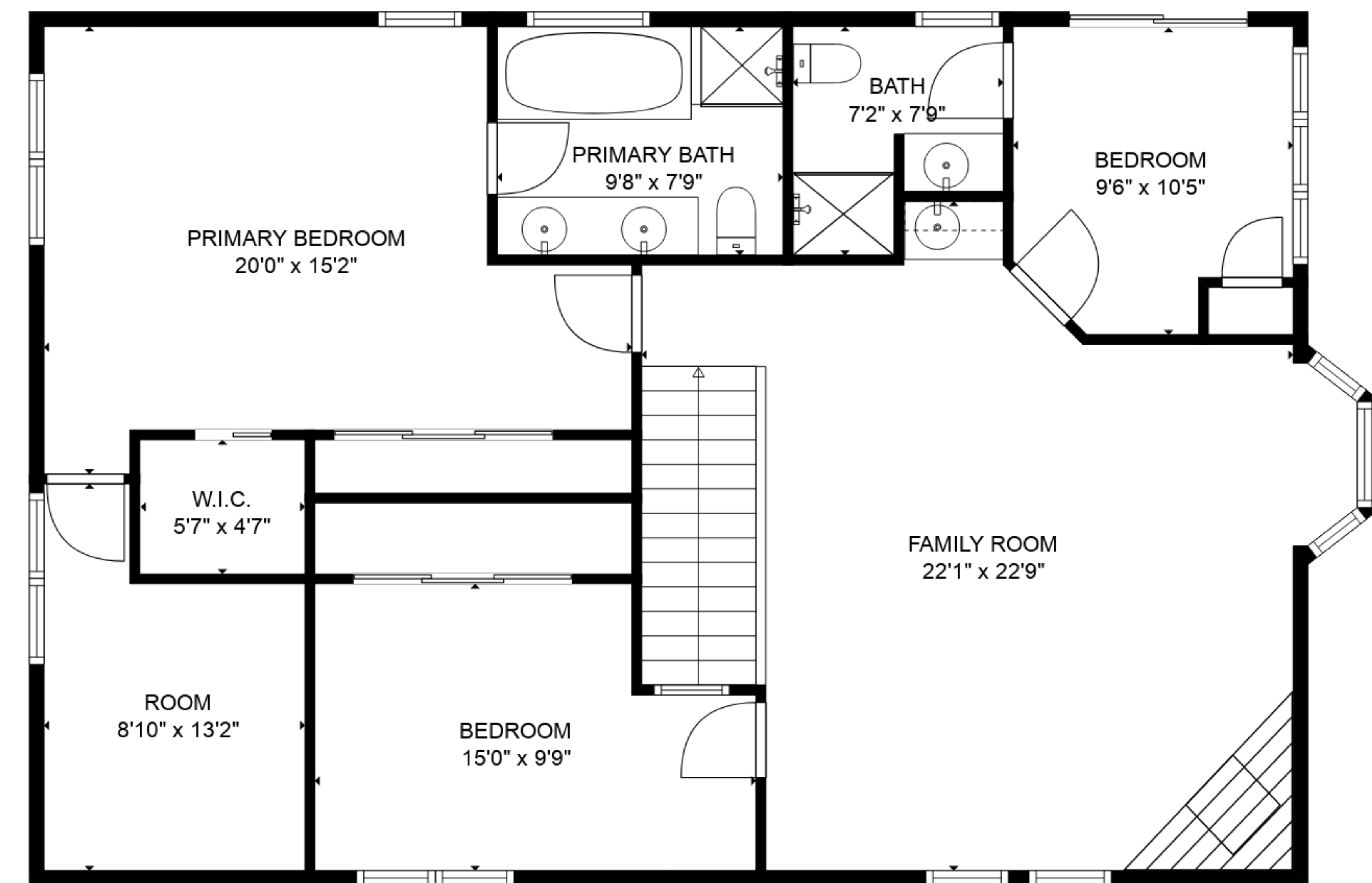
FLOOR 3
