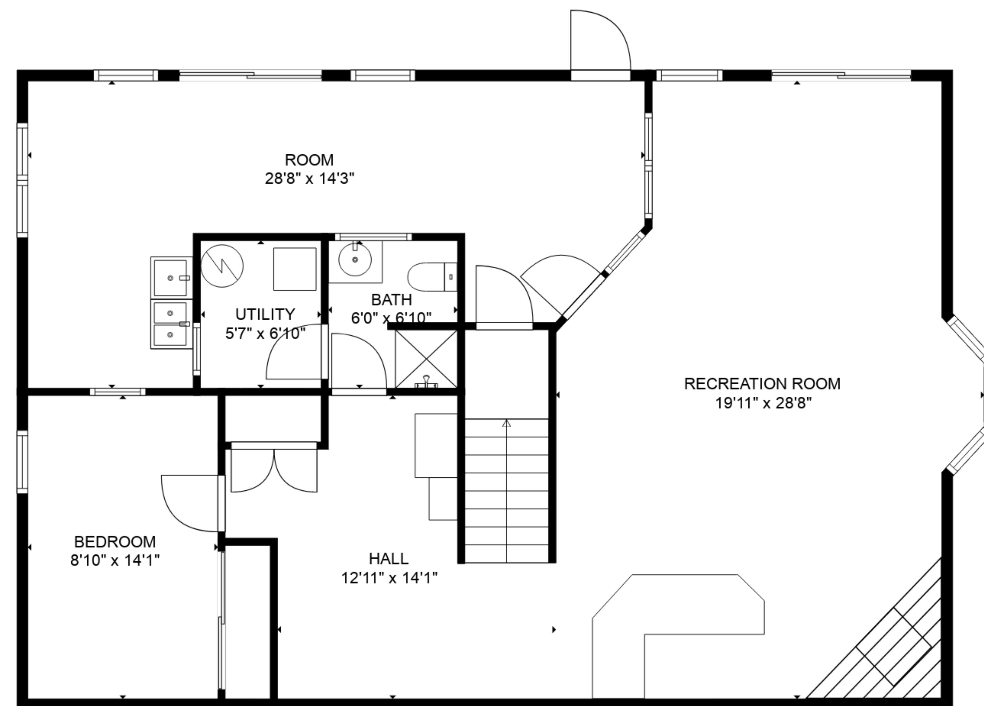
FLOOR 1
