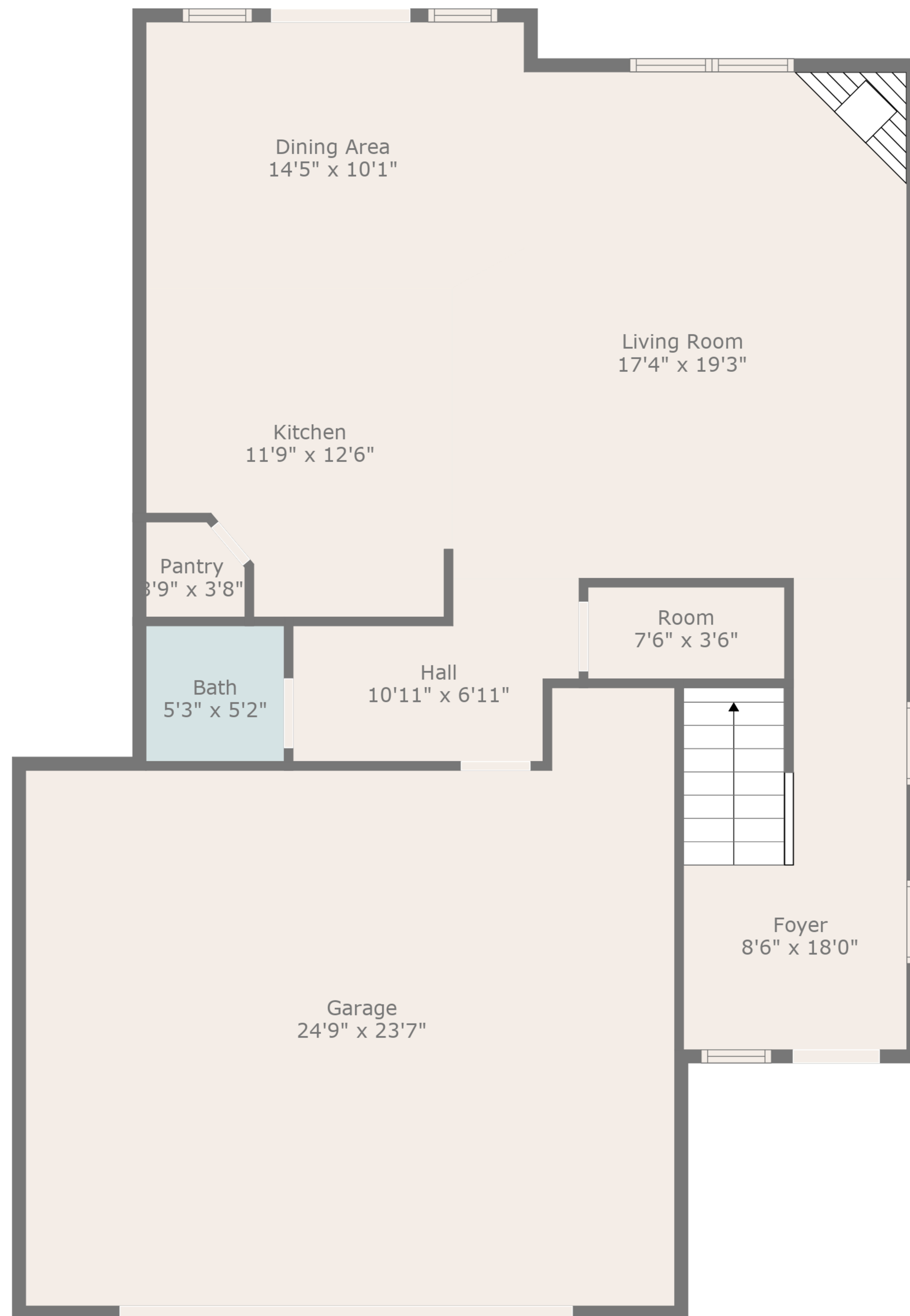
Floor 1
