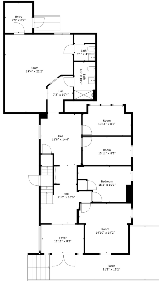
Floor 2
