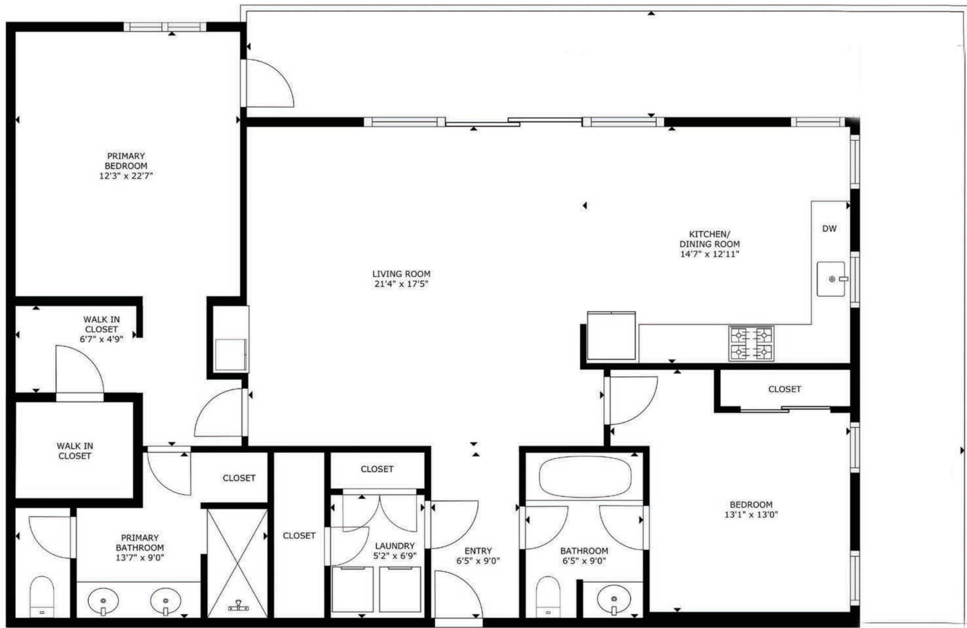
FLOOR PLAN
