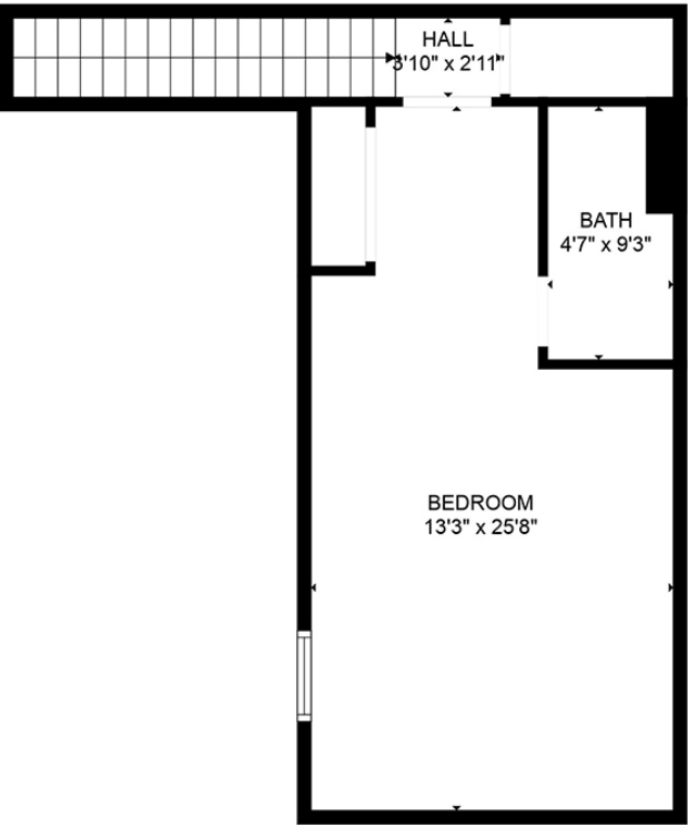
FLOOR 2
