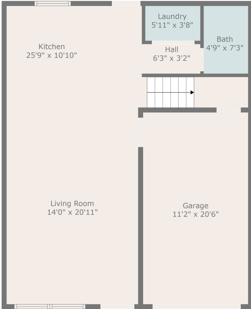
Floor 1
