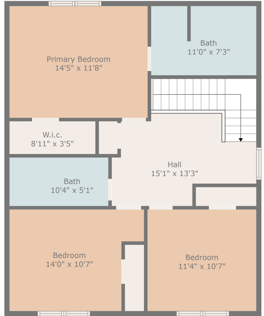
Floor 2
