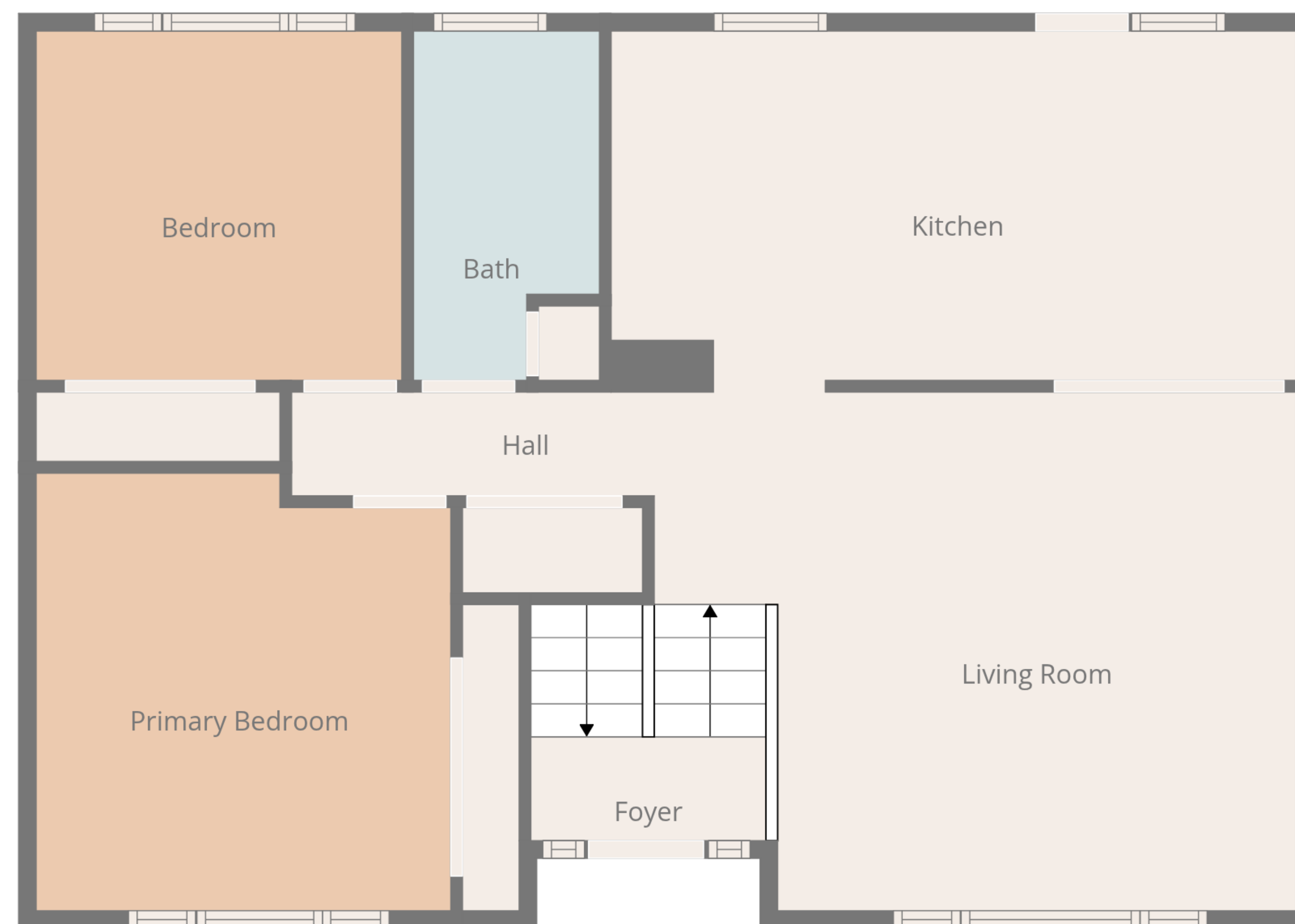
1st Floor
