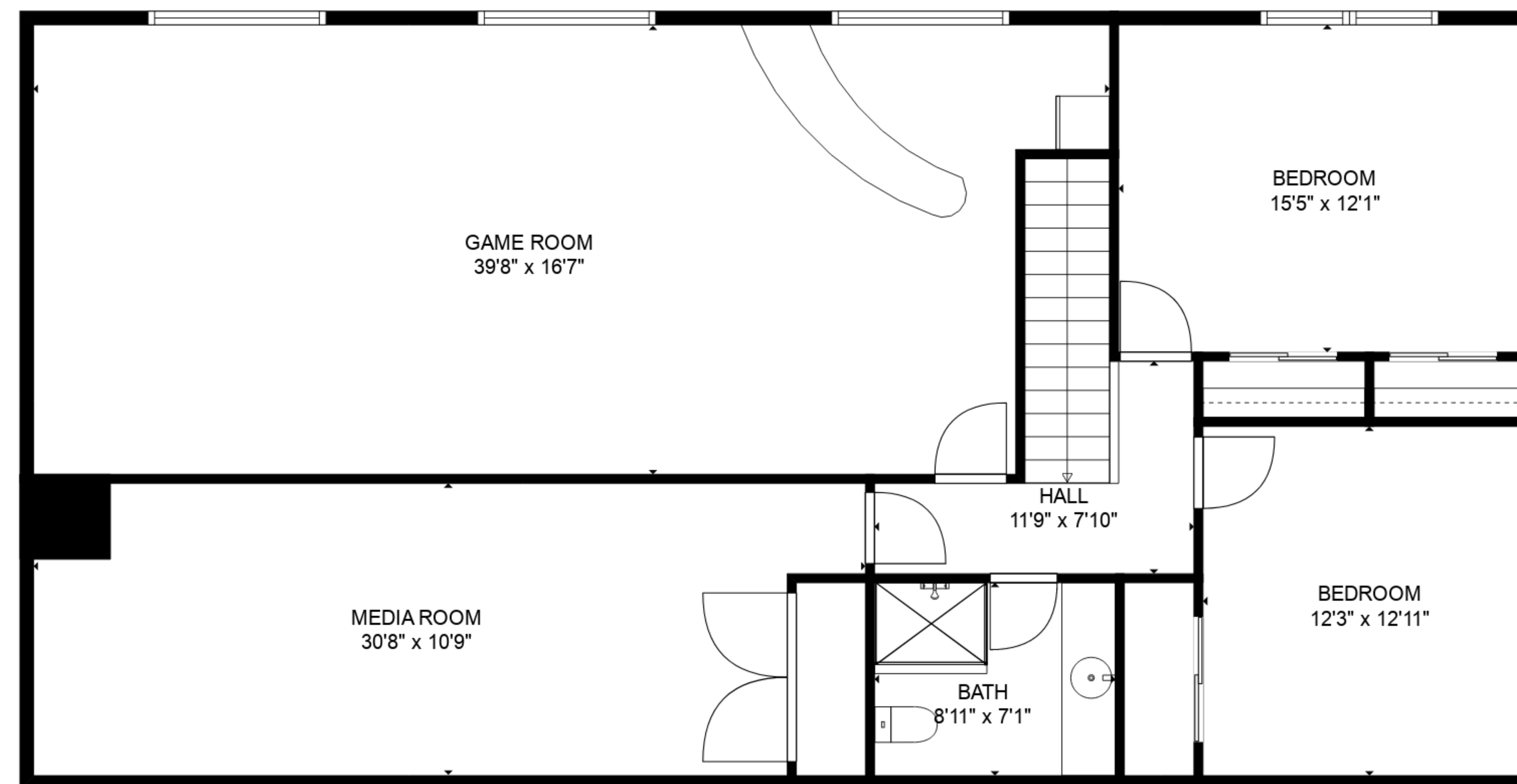
FLOOR 2
