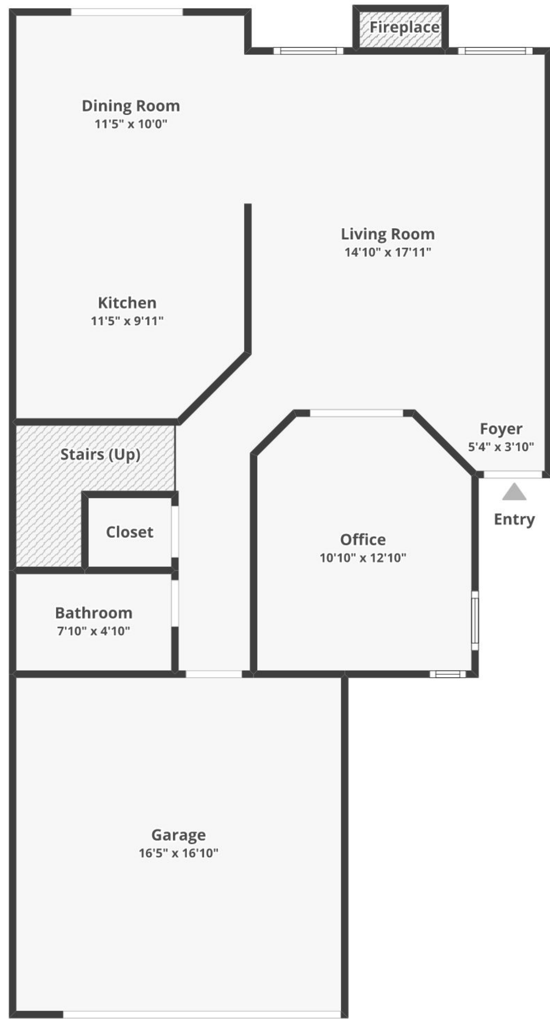
FLOOR 1
