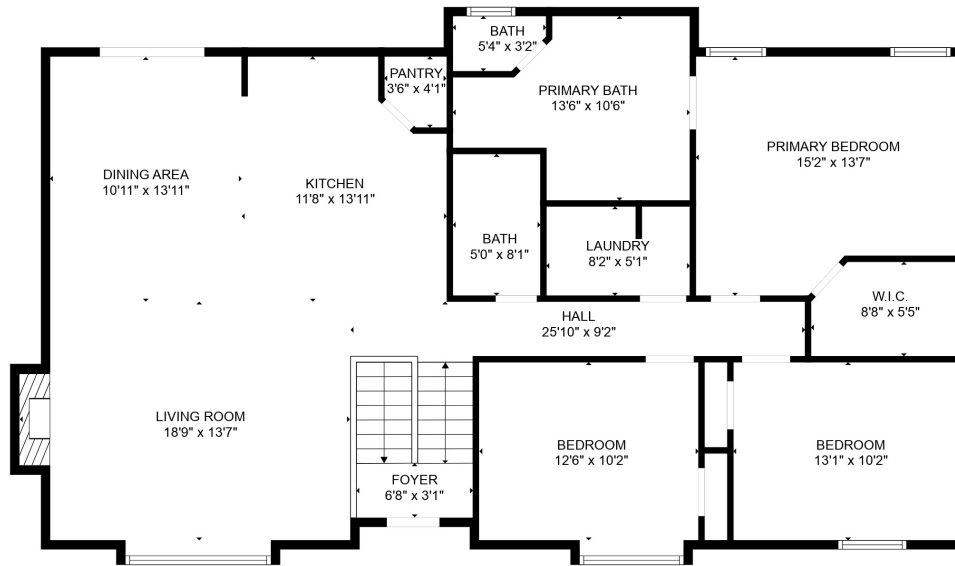
FLOOR 2
