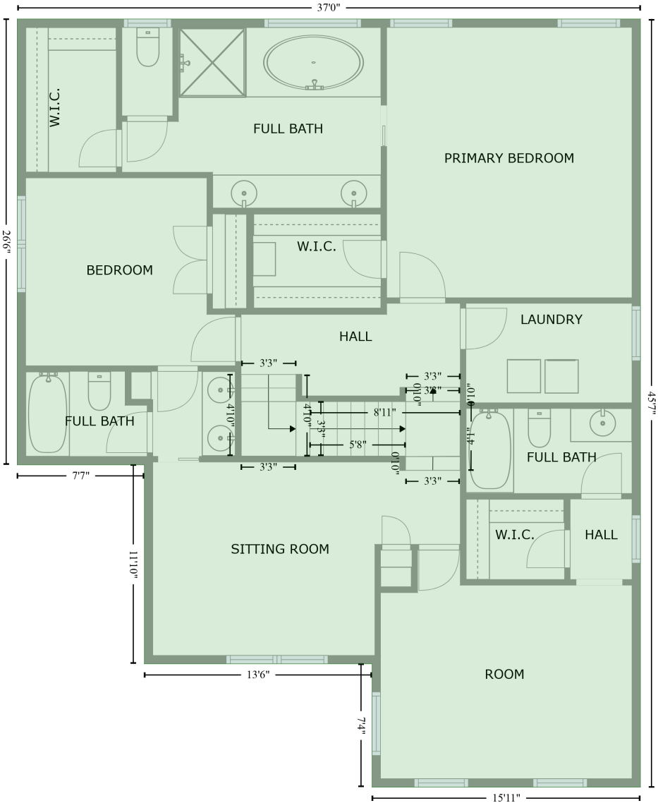
FLOOR 2 [AREA: 1443]
