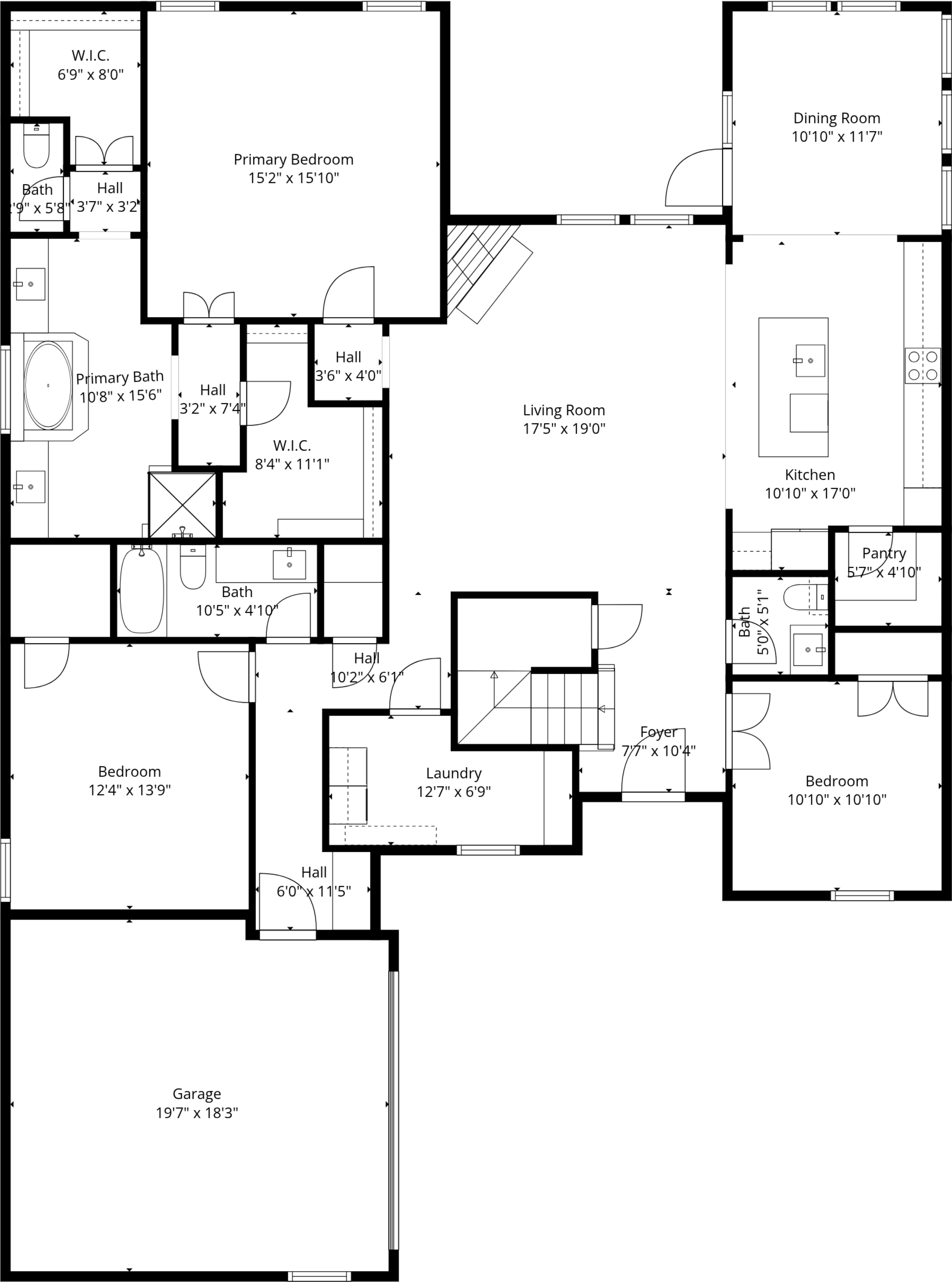
Floor 1
