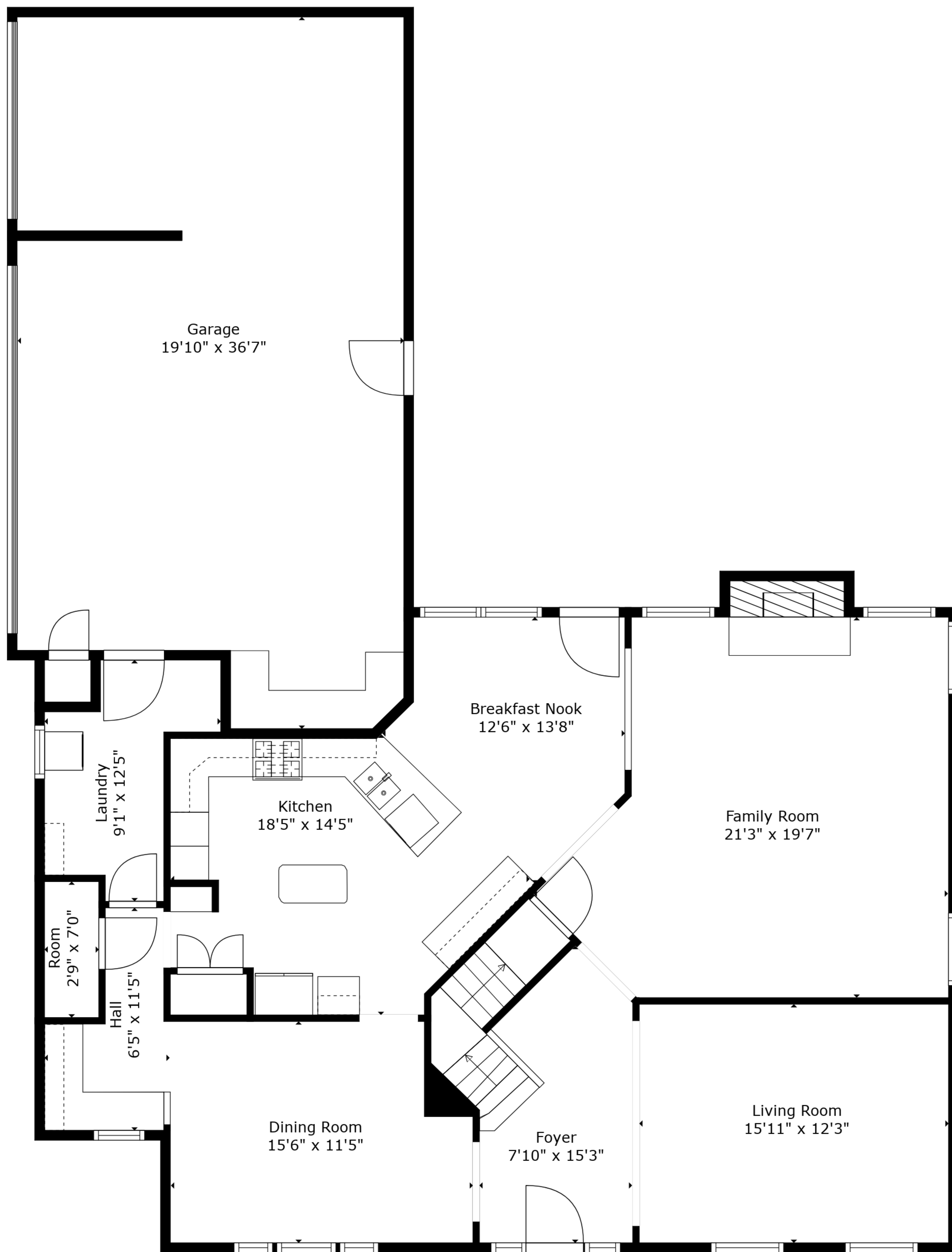
Floor 1
