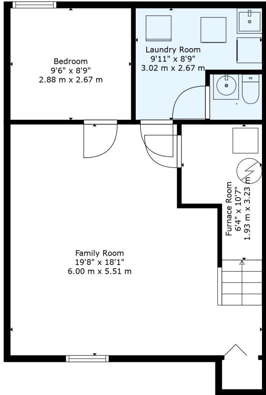
Floor 1
