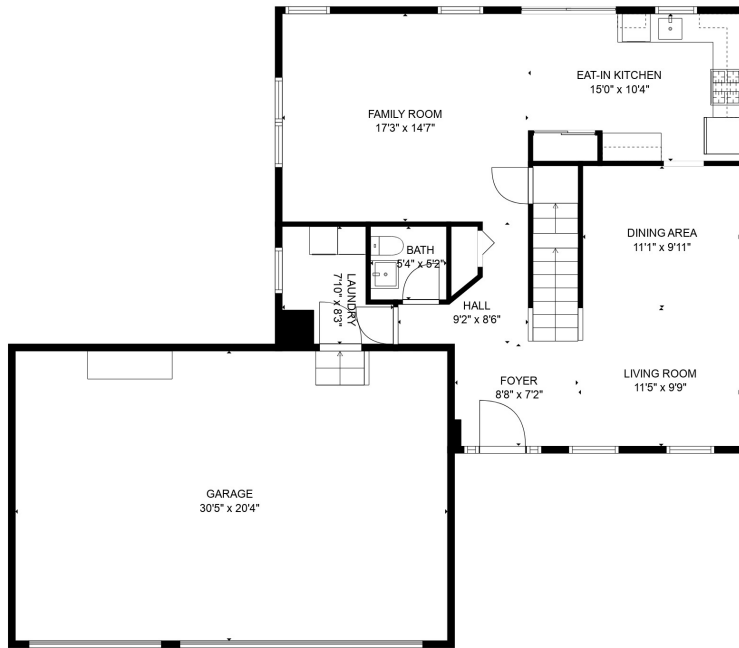
FLOOR 2
