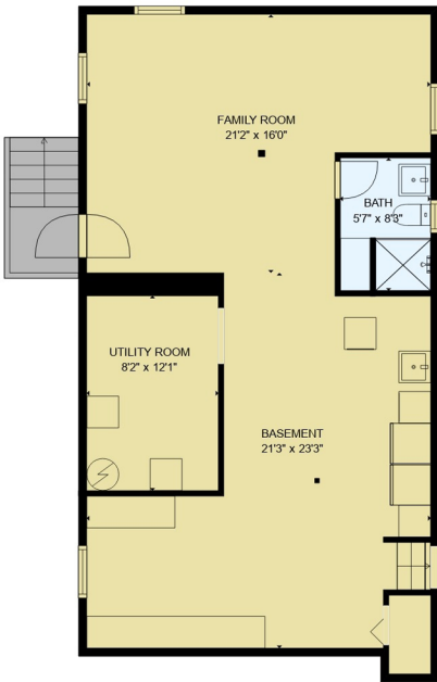
FLOOR 1
