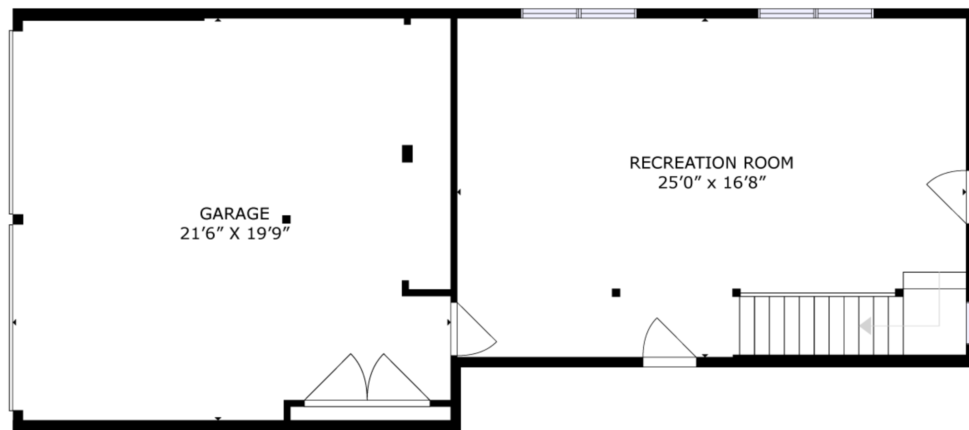
BASEMENT 1
