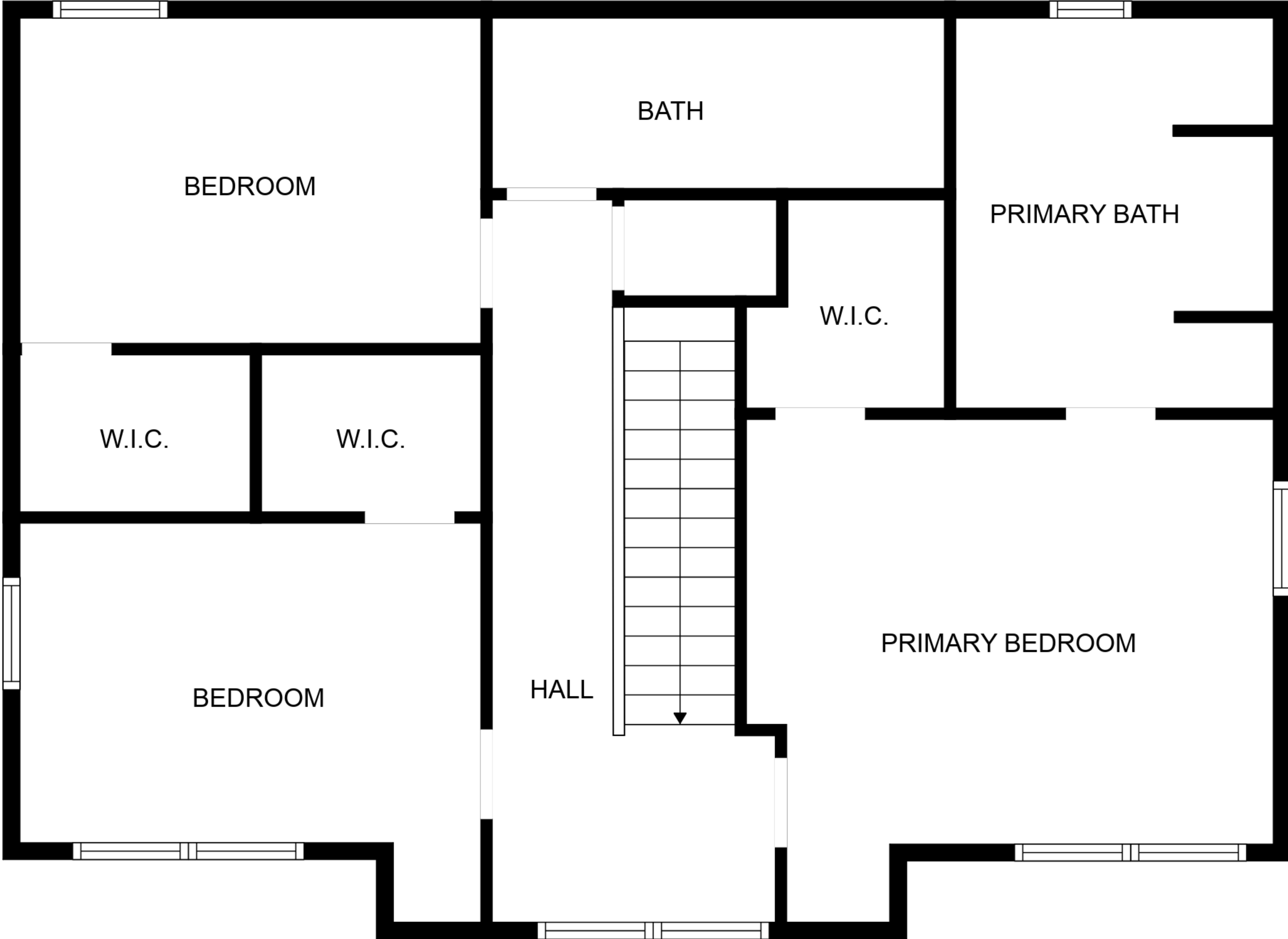
FLOOR 2
