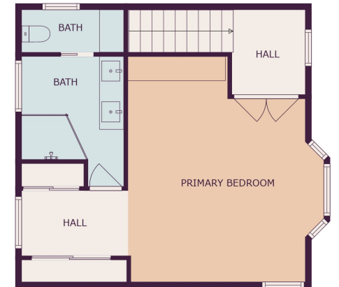
FLOOR 2
