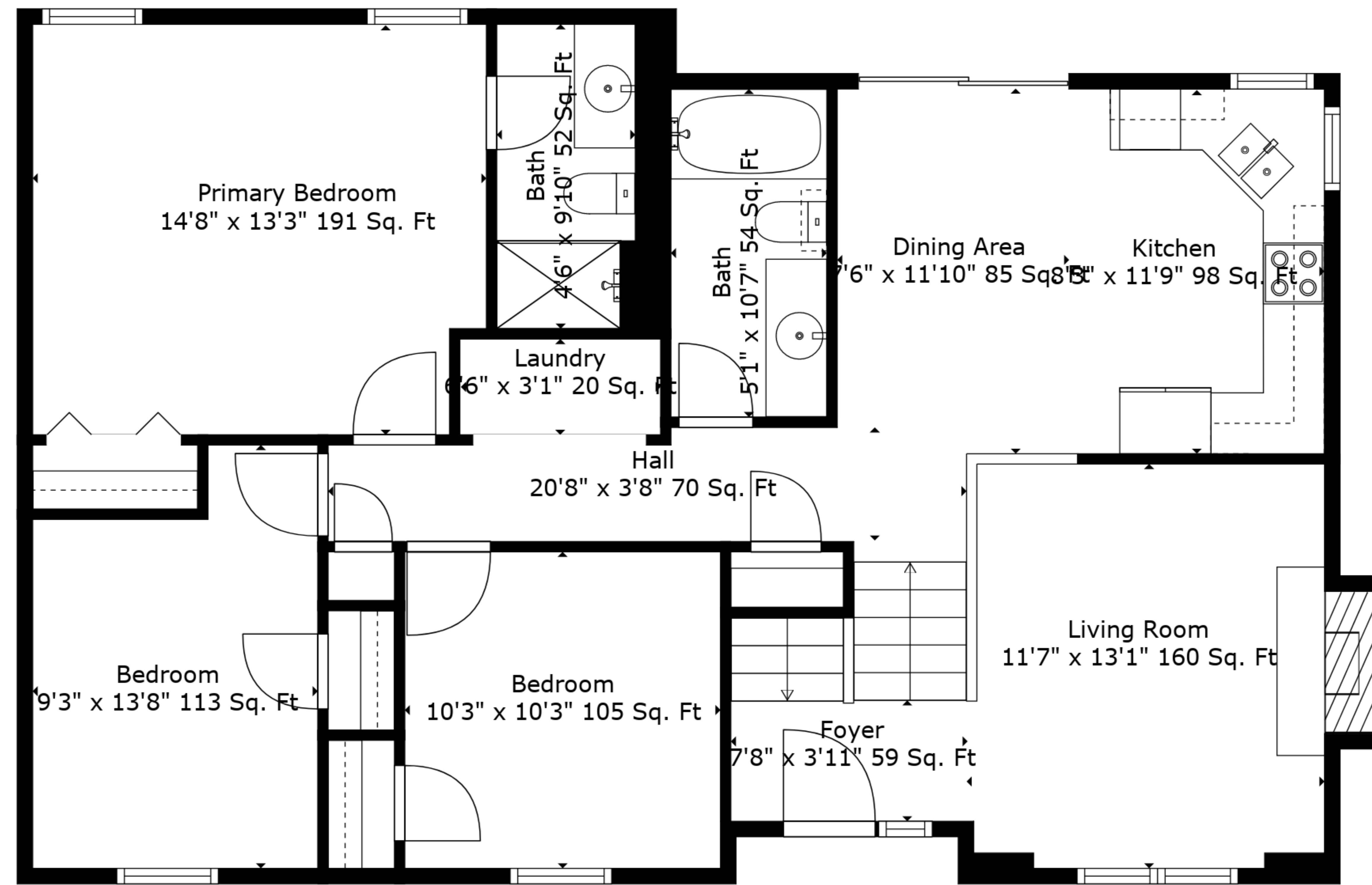
Floor 2
