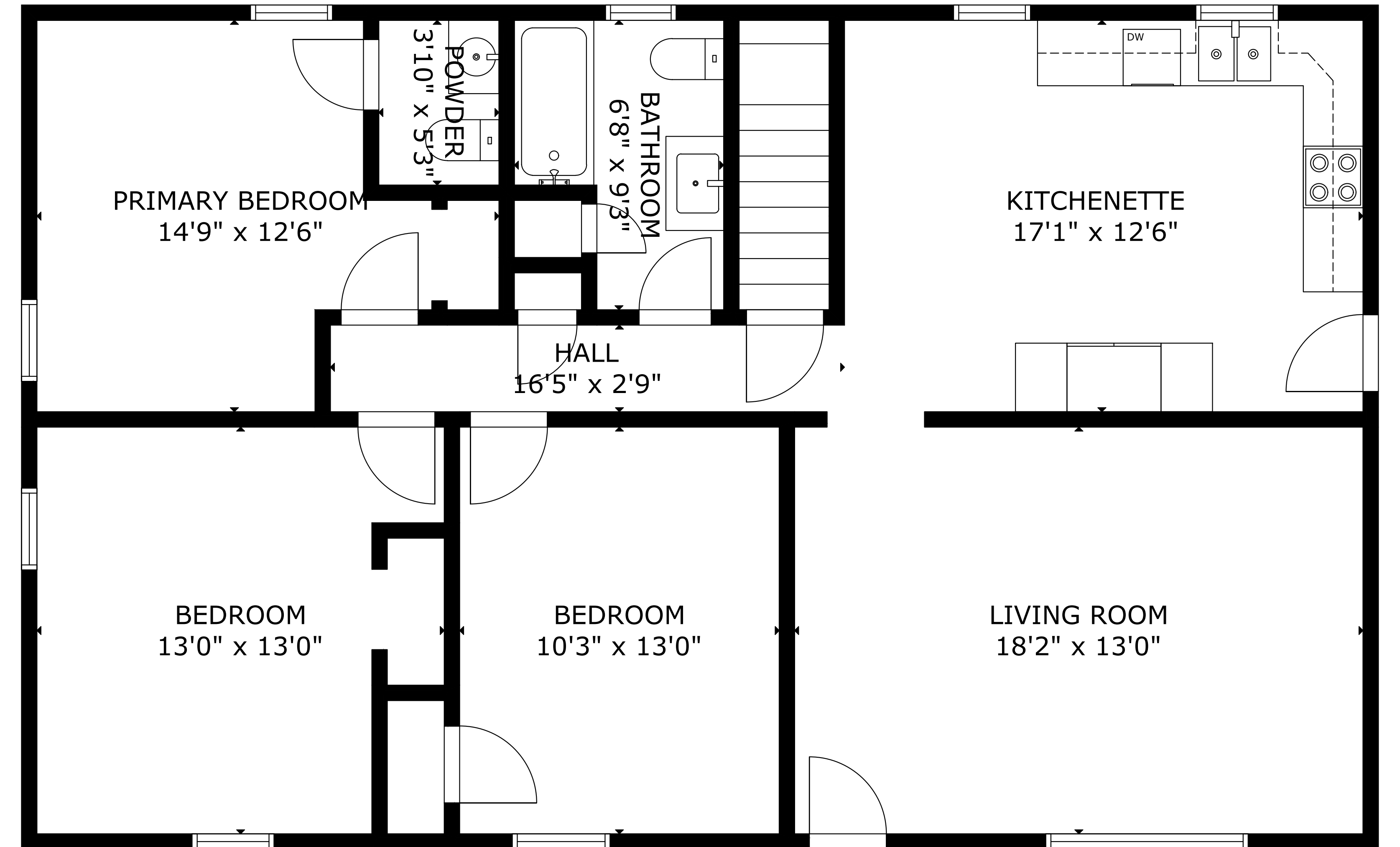
MAIN FLOOR
