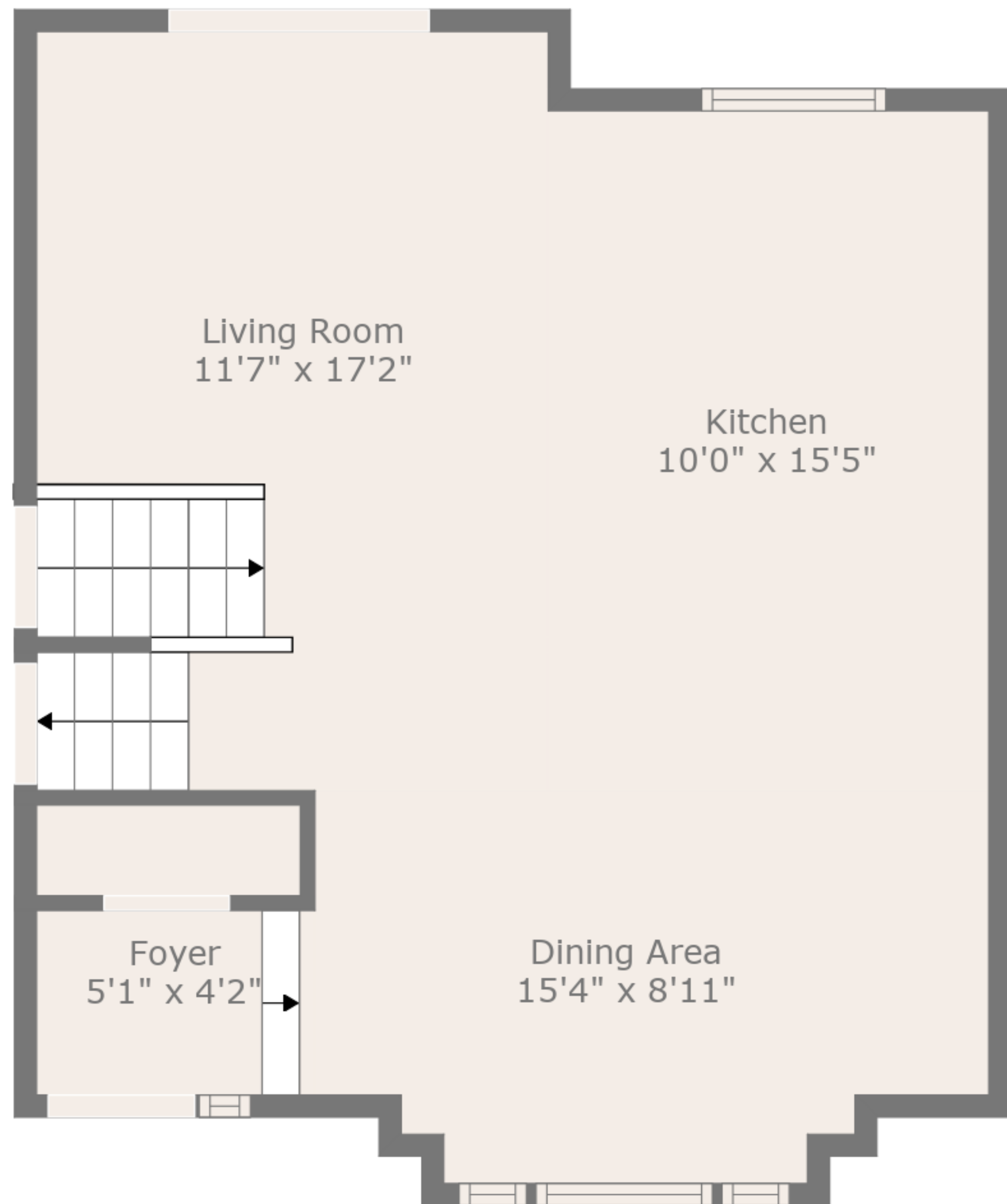
Floor 3
