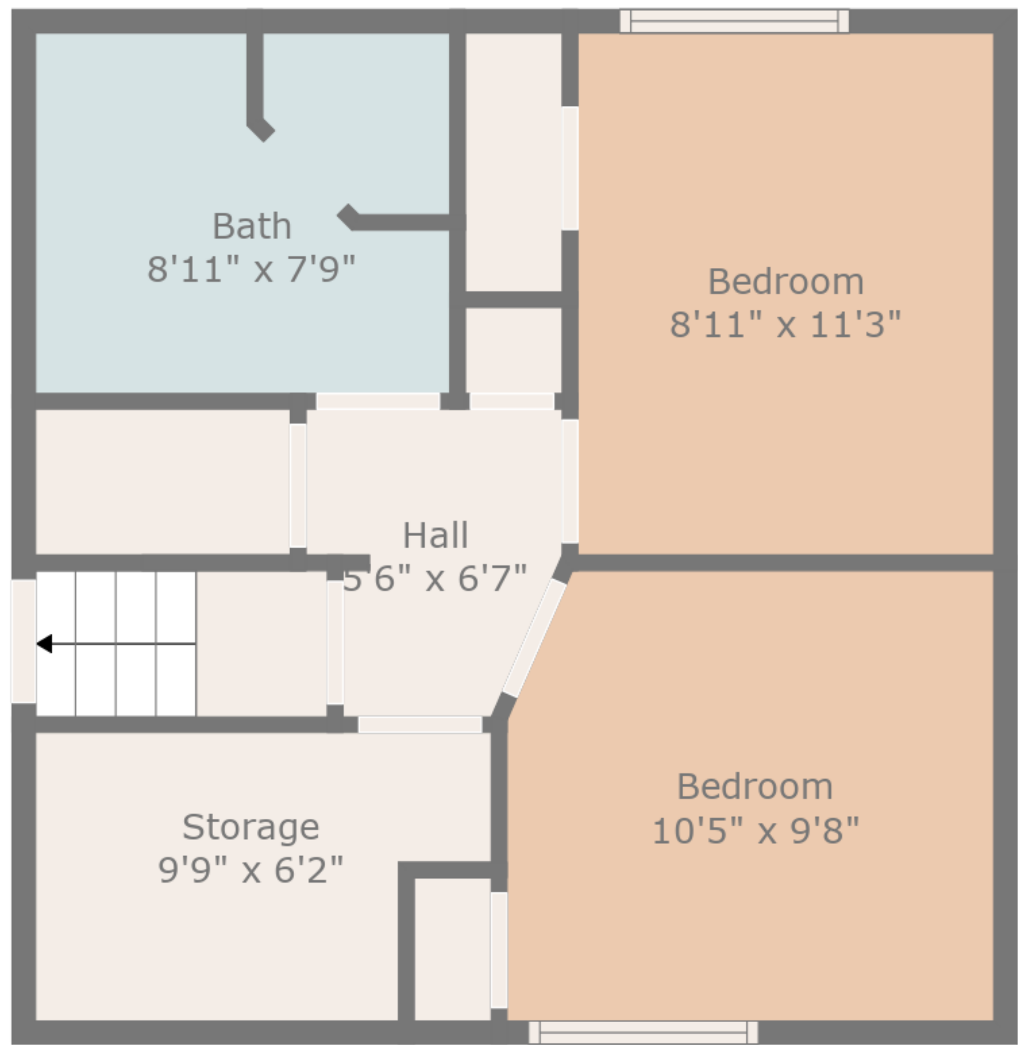
Floor 1
