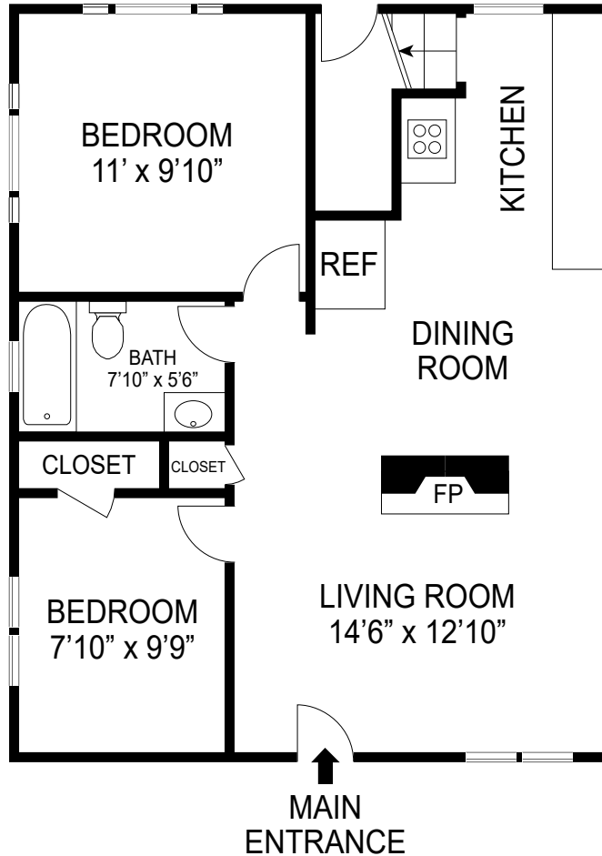
FIRST FLOOR 663 sqf
