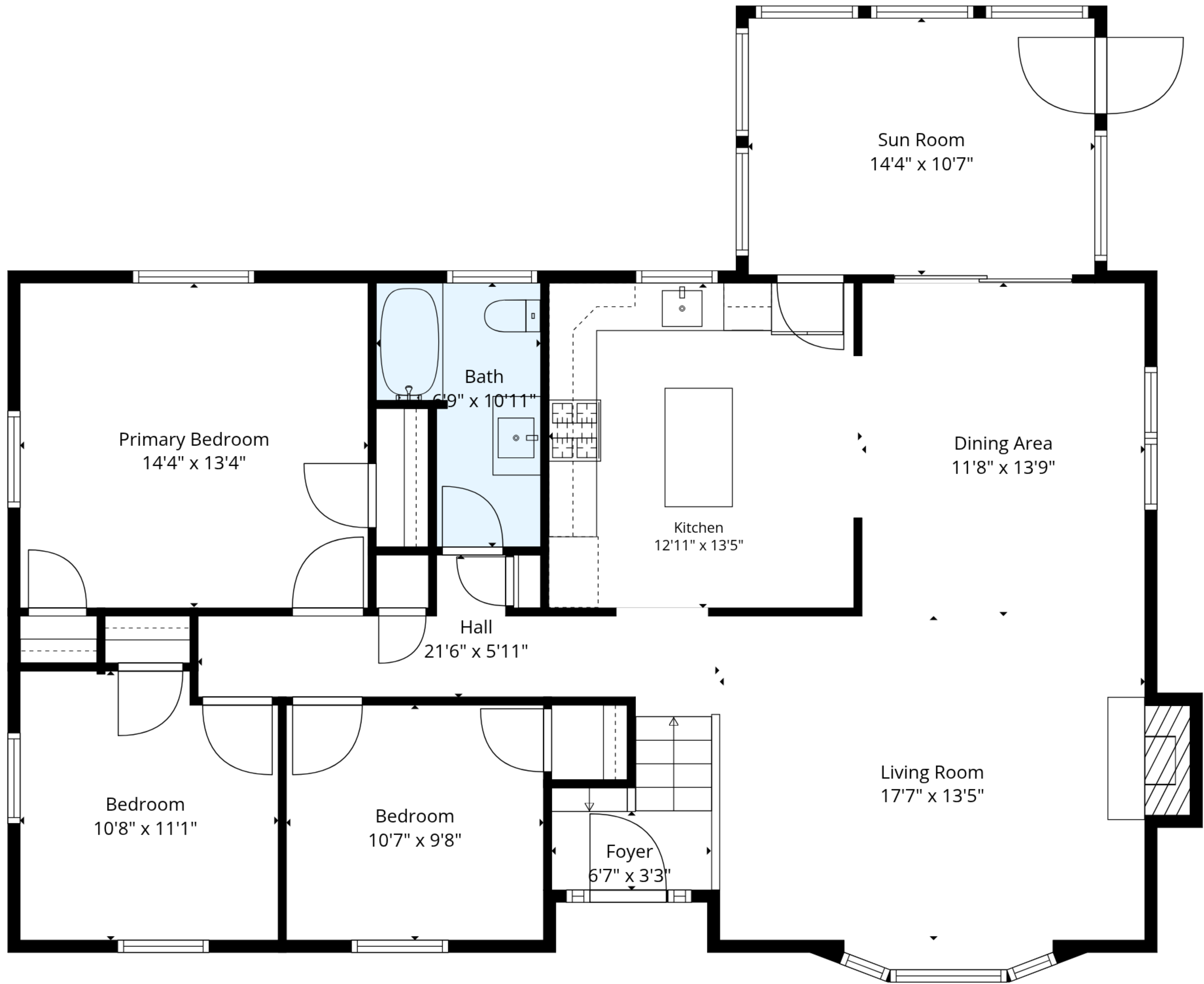
2nd Floor
