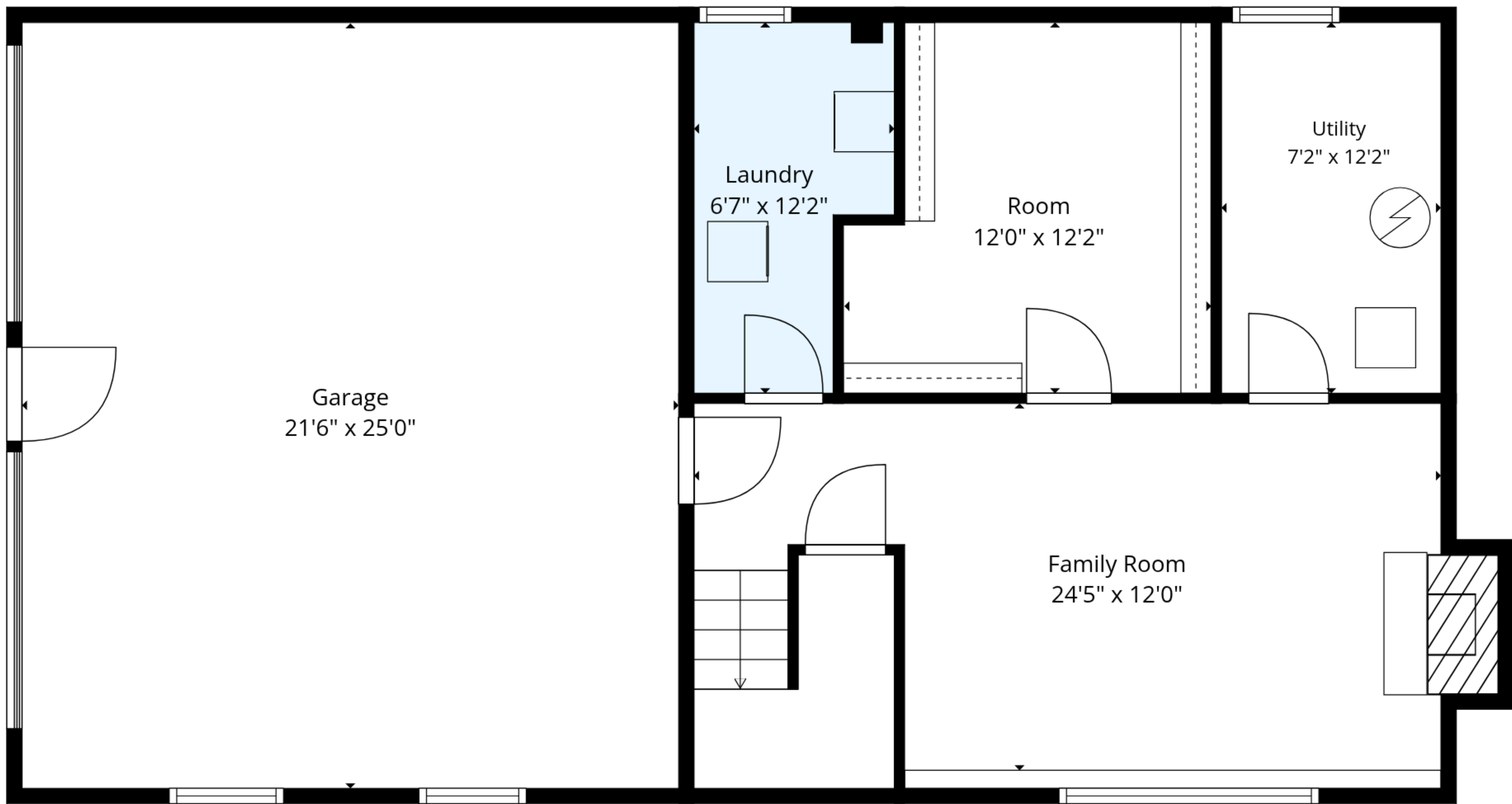
1st Floor
