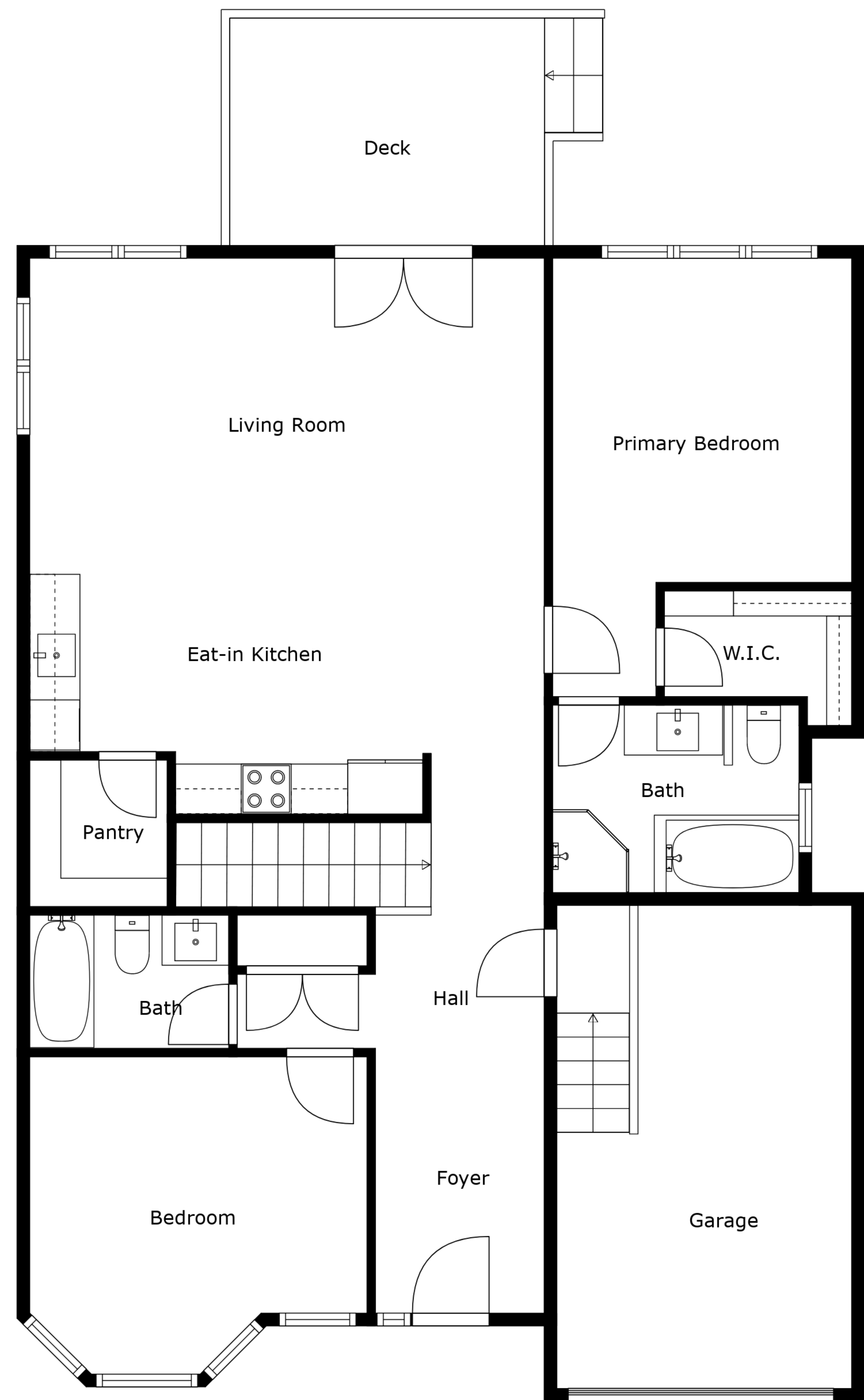
Floor 2
