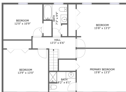
FLOOR 3
