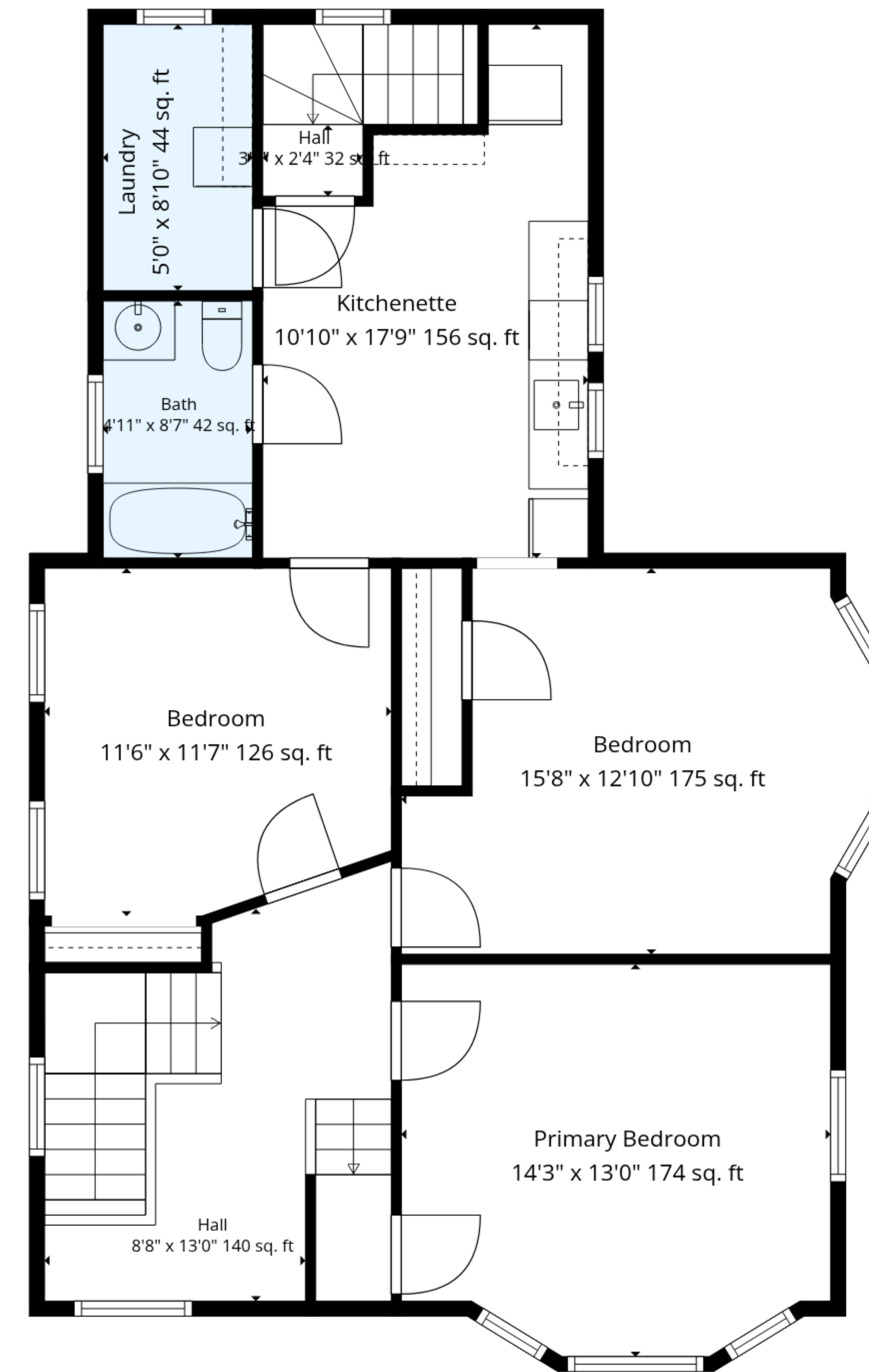
2nd Floor
