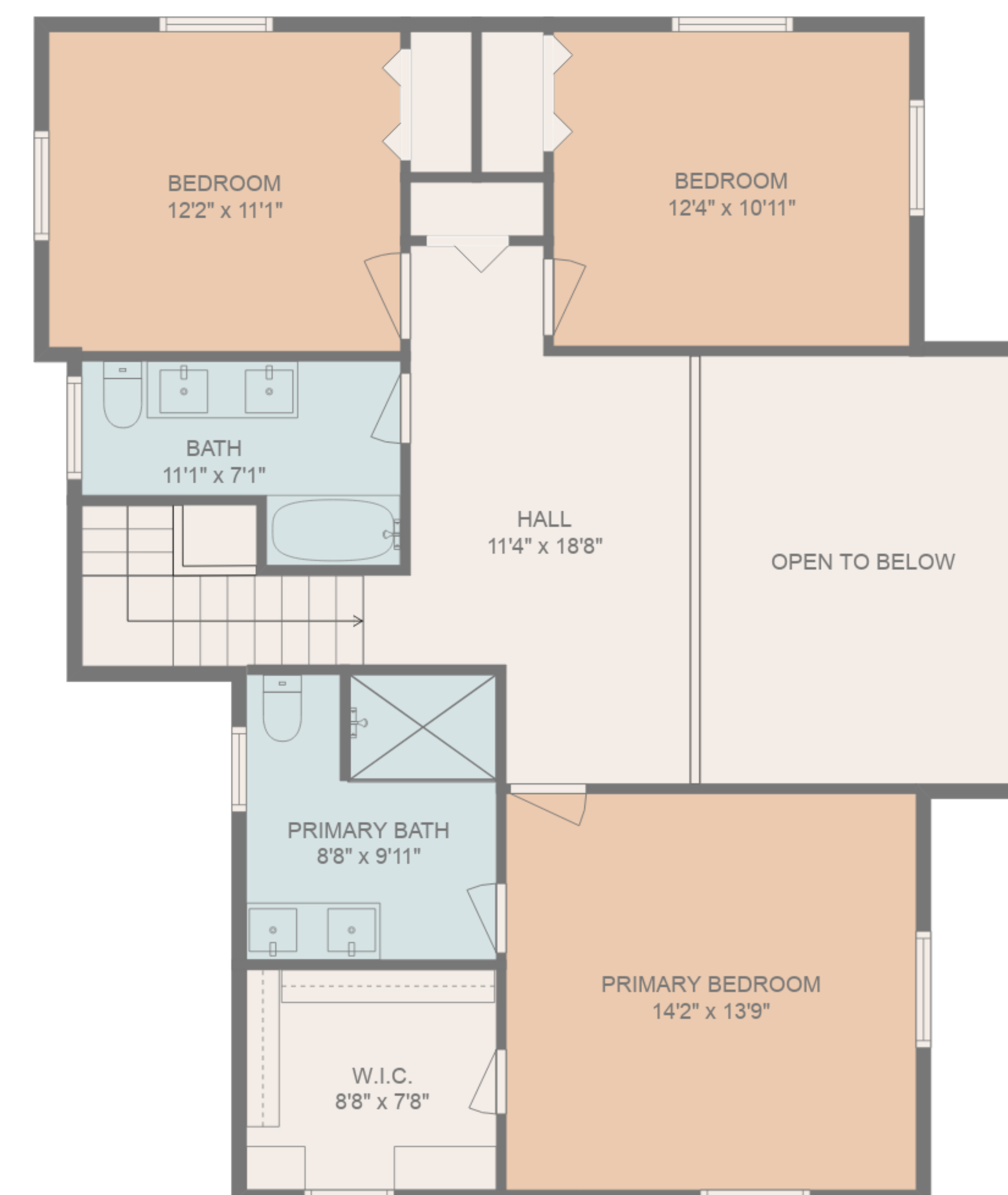
FLOOR 3
