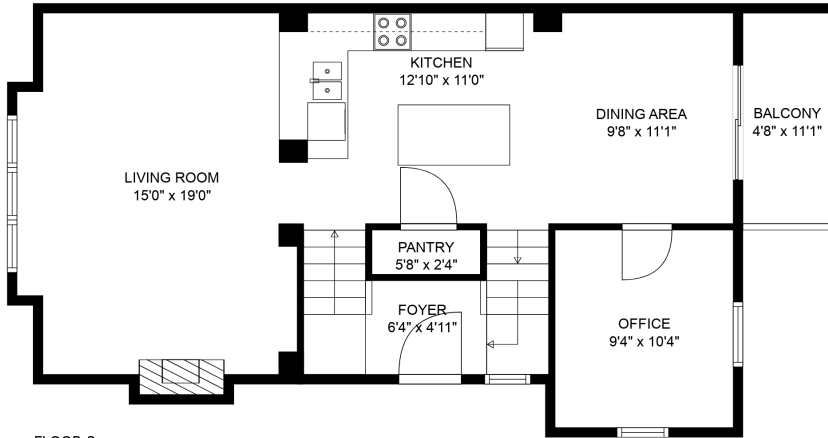
FLOOR 2
