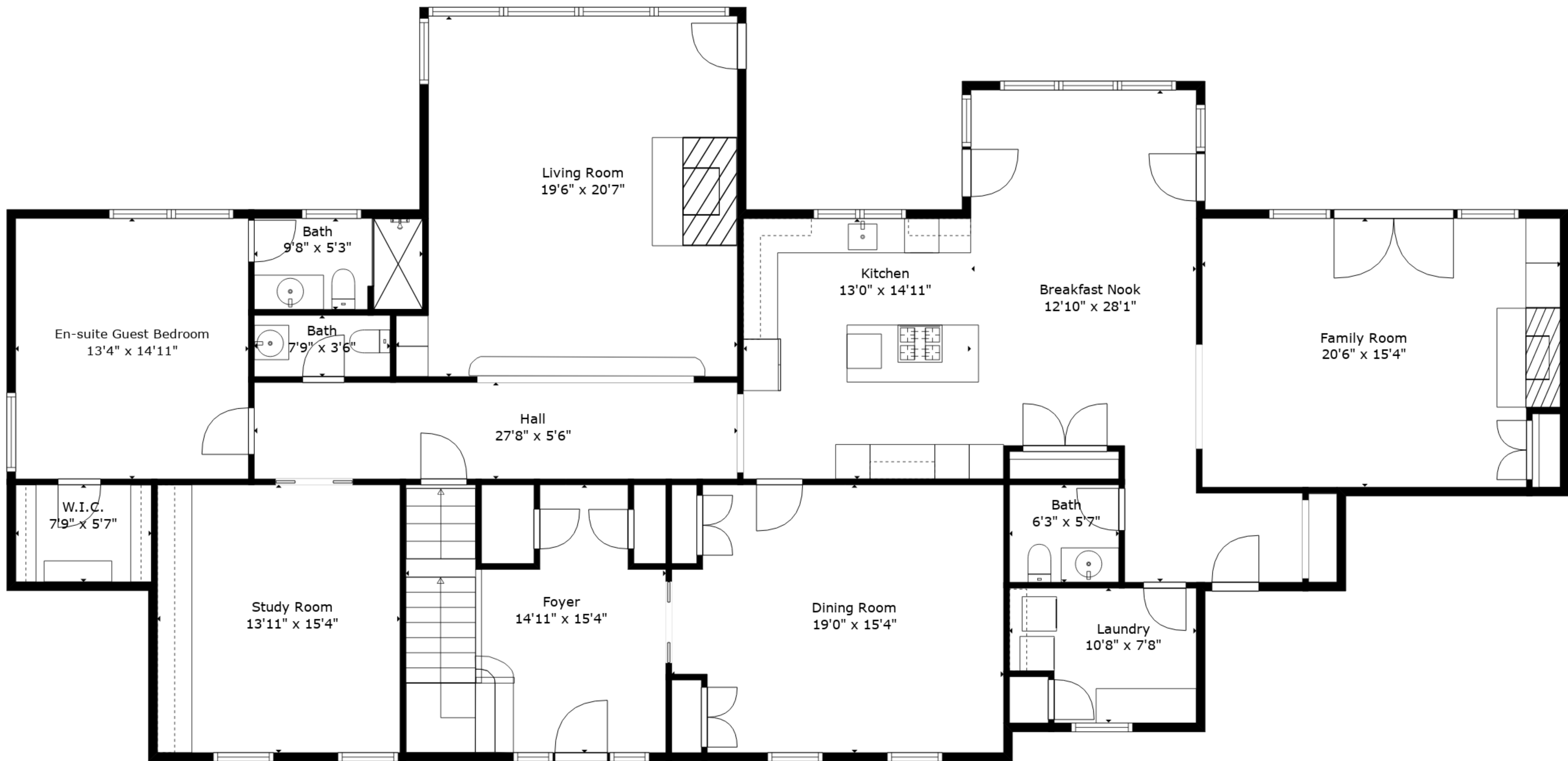
Floor 2
