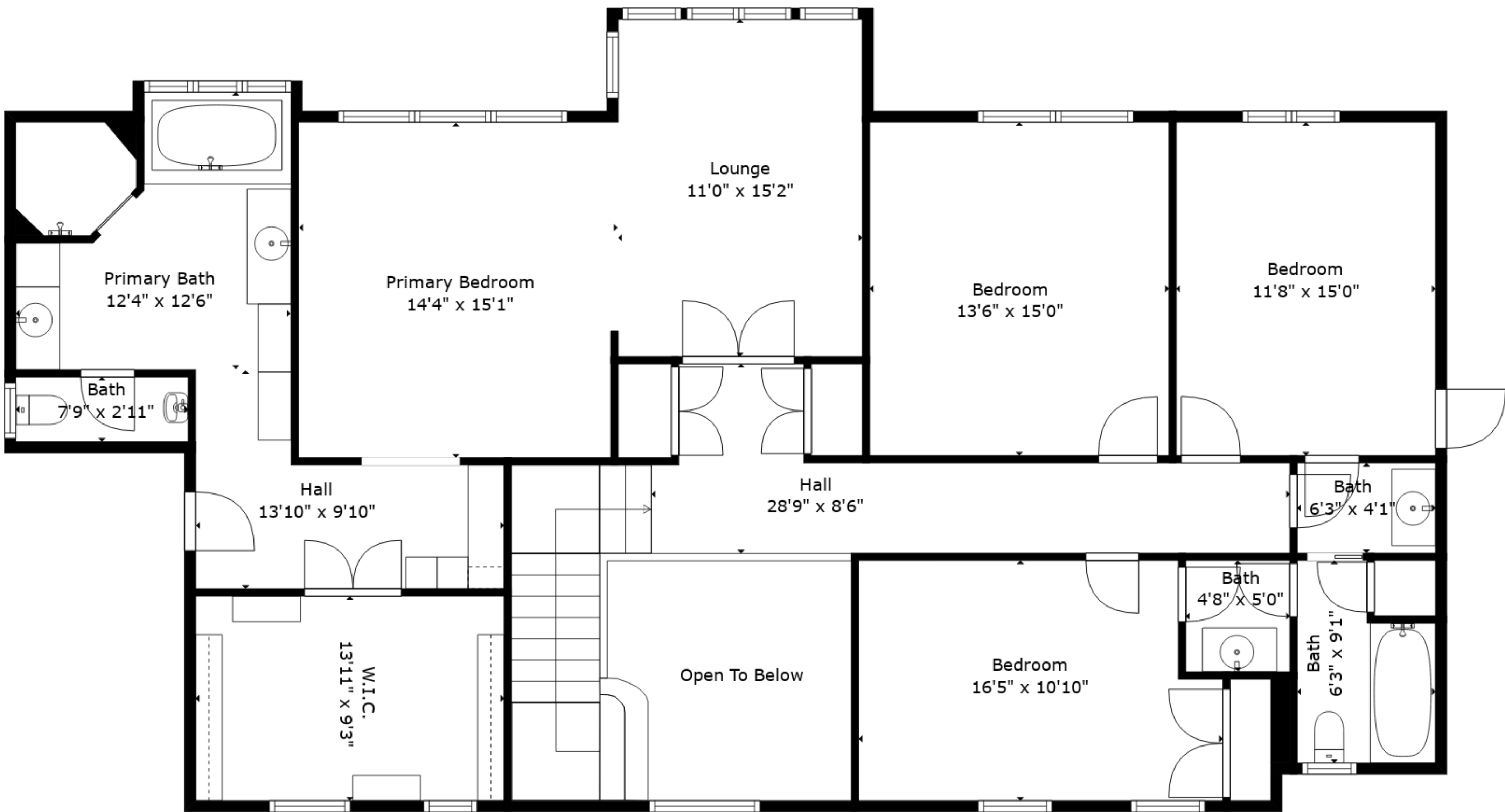
Floor 3
