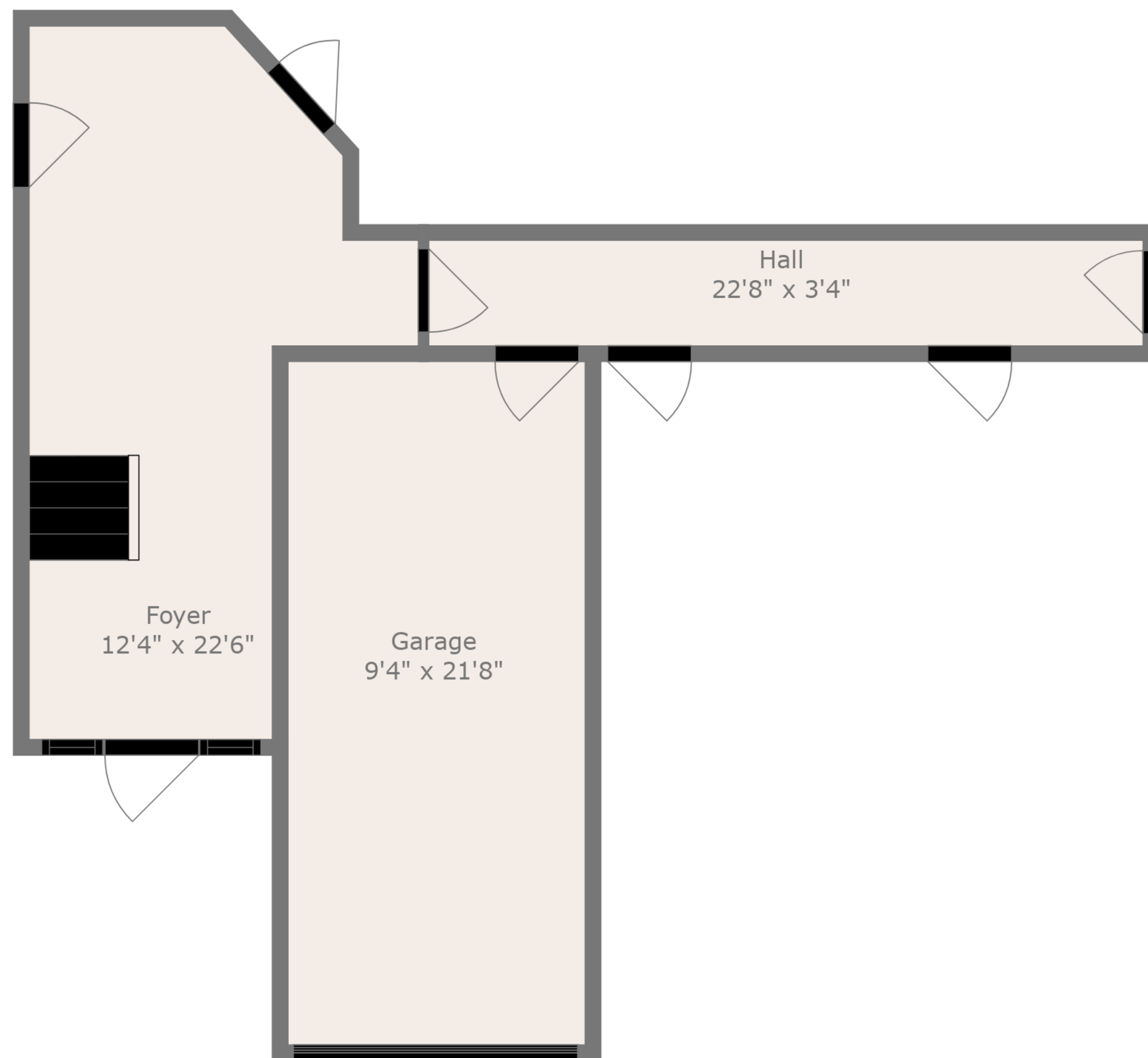
Floor 1
