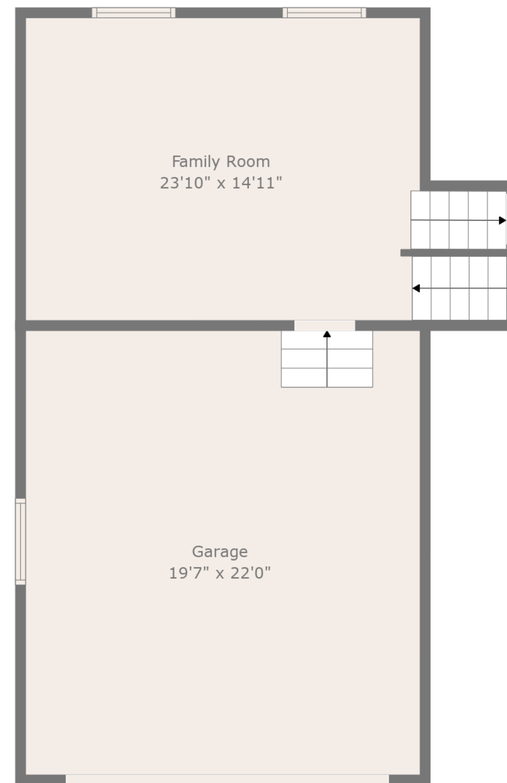
Floor 2
