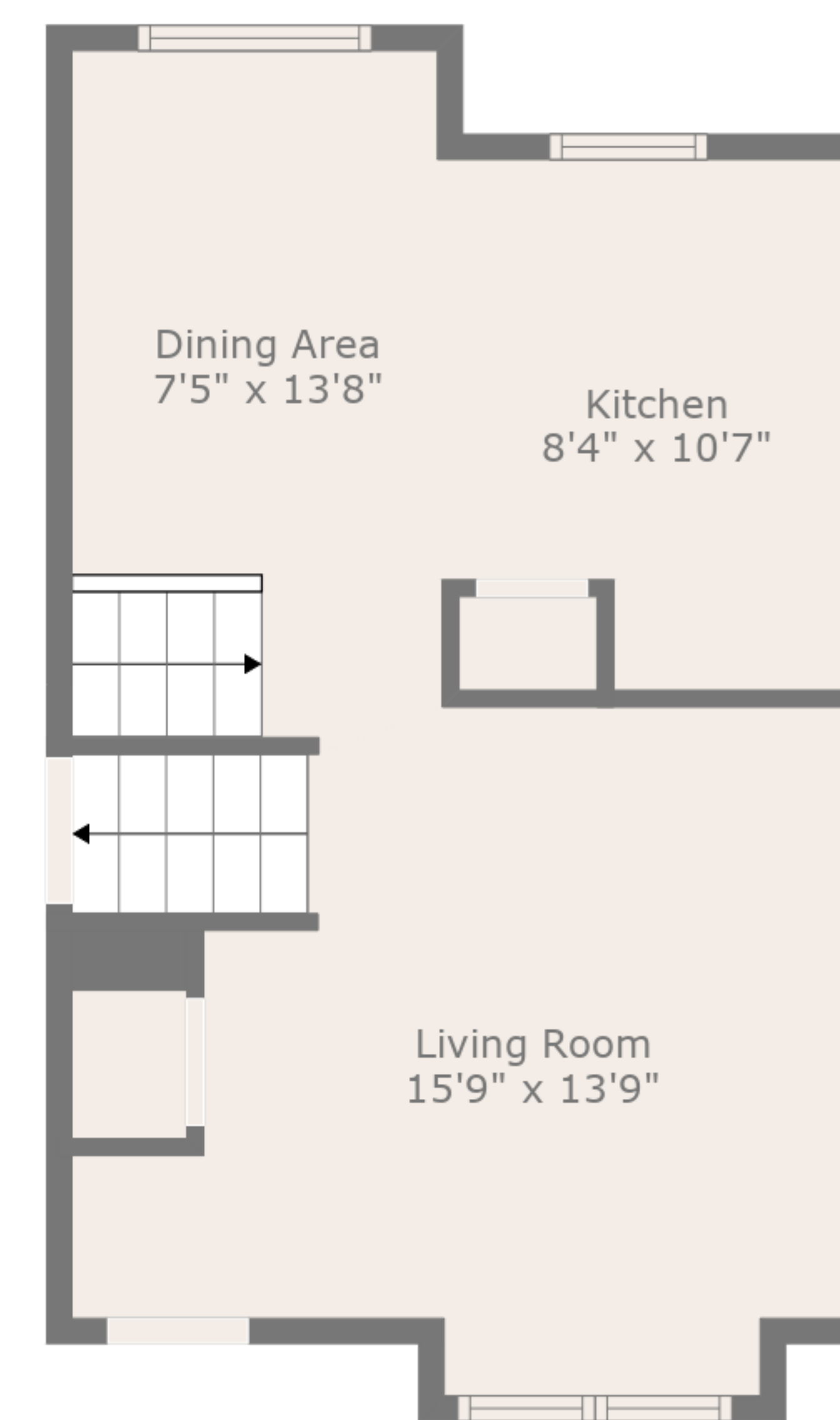
Floor 3
