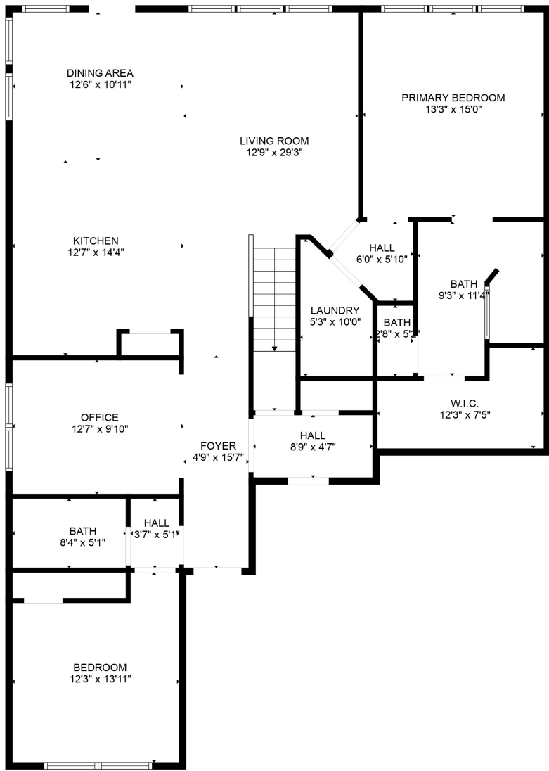
FLOOR 1
